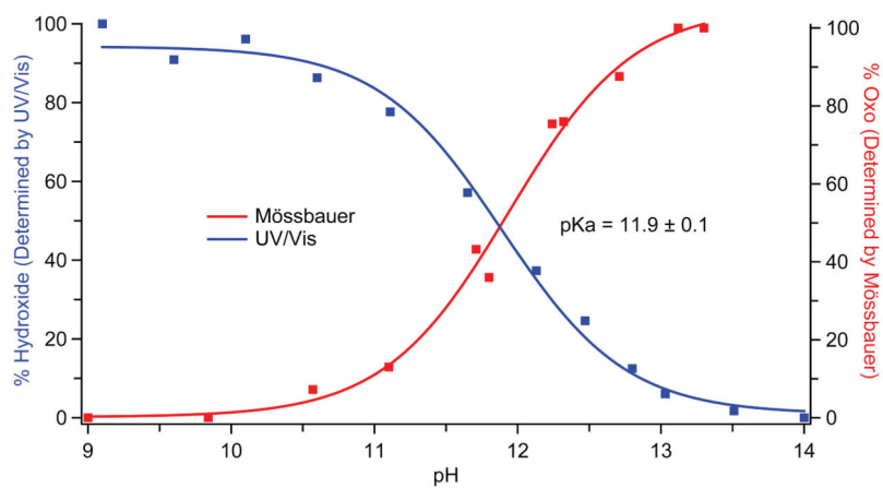
Fig. 4. pH titration curves for CYP158-II. Data obtained from stopped-flow UV/Visible (blue) and Mössbauer spectroscopies (red) yield the same pKa value of 11.9. UV/Visible data points were obtained from the change in absorbance at 423 nm (Fig. 2). Mössbauer data points were obtained from the ratio of the areas of the iron(IV)oxo and iron(IV)hydroxide subspectra (fig S2).
