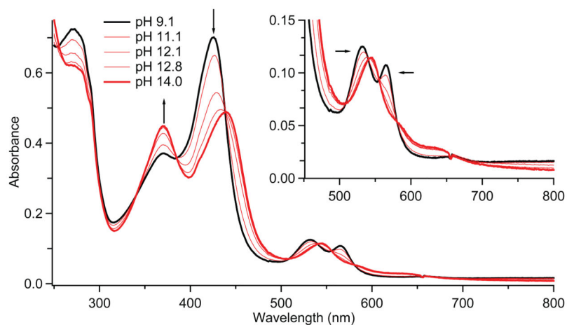
Fig. 2. UV/Visible spectra of CYP158-II at varying pH. Samples were prepared in a double-mix stopped-flow experiment. 30 \mu M ferric CYP158 (10 mM Tris-HCl, pH 9.0) was first mixed with 150 \mu M m -CPBA and held until maximum formation of CYP158-II was achieved (2.5 seconds). This solution was then mixed with a strongly buffered solution (containing 200 mM phosphate, 200 mM carbonate, pH adjusted with KOH) to obtain the desired final pH. Mixing was 1:1:1. The inset shows a magnification of the 450–800 nm region.
