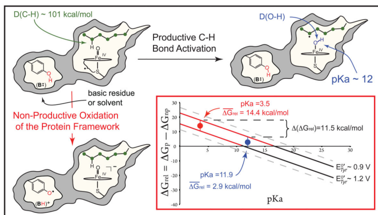
Fig. 1. Productive and non-productive pathways for compound I decay. During productive C-H bond activation, compound I (a ferryl-radical species) abstracts hydrogen from substrate to yield compound II (an iron(IV)hydroxide complex) and a substrate radical. The non-productive pathway shown involves the oxidation of a tyrosine residue contained within the protein framework, with the phenolic proton being transferred to B: , a basic residue or solvent molecule, upon tyrosine oxidation. The inset shows the relative free energies ( \Delta G_{\text{rel}} , Eq. 5) for the productive and non-productive pathways as a function of the compound II pKa for the range of aqueous tyrosine potentials. When \Delta G_{\text{rel}} is negative, the productive pathway is thermodynamically preferred. As a result of the \pm 2 kcal/mol error in Eq. 2, a small range of tyrosine potentials could yield a given \Delta G_{\text{rel}} . The uncertainty in the solid lines as a result of this error is \pm 0.1 V.
