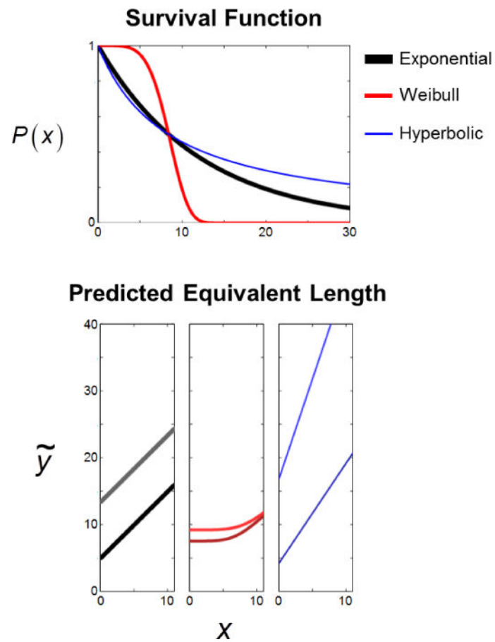
Figure 2. Illustration of three classes of survival models
