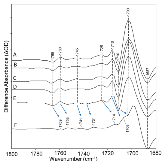
Figure 7. Spectra from Figure 2 over the 1680–1800 \text{cm}^{-1} region: (A) CaChR1 in H 2 O, (B) CaChR1 in H 2 O regenerated with A1 retinal, (C) CaChR1 in H 2 O regenerated with A2 retinal, (D) CaChR1 in H 2 O regenerated with [15- 13 C,15- 2 H]retinal, (E) CaChR1 in H 2 O regenerated with [14,15- 2 H 2 ]retinal, and (F) CaChR1 in D 2 O. Arrows indicate shifts of difference bands due to H–D exchange. Y axis markers are approximately 0.5 mOD for all spectra. See the discussion in the Supporting Information regarding results shown in spectra B–F.
