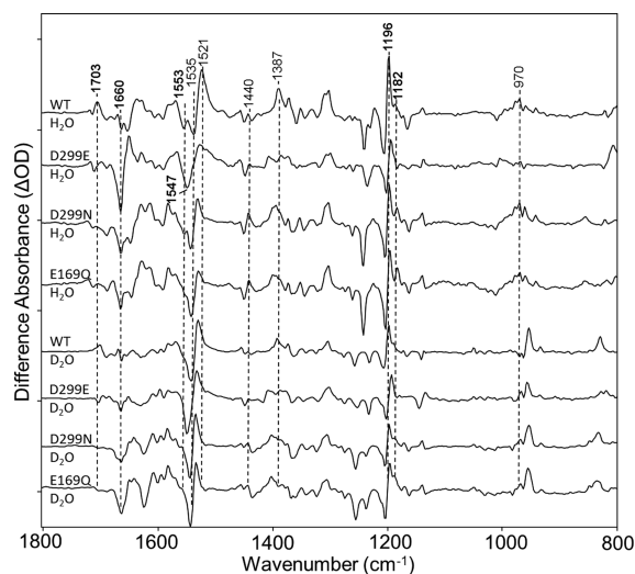
Figure 8. Comparison of CaChR1 and the D299N, E169Q, and D299E mutants over the region from 800 to 1800 \text{cm}^{-1} . The top four spectra were recorded in H 2 O and the bottom four in D 2 O. All spectra were acquired as described previously. Peaks labeled in bold are discussed in the text. Y axis markers are approximately 3 mOD for WT, 2 mOD for D299E, 2.5 mOD for D299N, and 1 mOD for E169Q. For detailed H–D exchange and site-directed mutagenesis procedures, see Materials and Methods.
