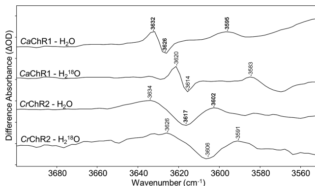
Figure 5. Comparison of the weak hydrogen bonding region from 3550 to 3700 \text{cm}^{-1} for CaChR1 and CrChR2 in H 2 O and H 2 18 O at 80 K. Peaks labeled in bold are discussed in the text. Y axis markers are approximately 0.1 mOD for both CaChR1 spectra and 0.05 mOD for both CrChR2 spectra. For detailed H 2 18 O exchange procedures as well as spectral acquisition parameters, see Materials and Methods.
