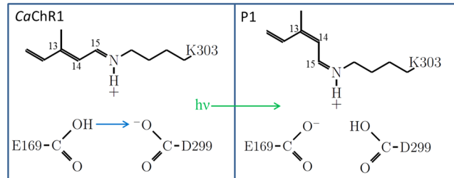
Figure 10. Schematic model showing Glu169 and Asp299 residues that interact with each other through a hydrogen bond formed by the carboxylic acid group of Glu169 and carboxylate group of Asp299. These residues together function as a counterion for the positively charged SB present in the unphotolyzed state of CaChR1 . During the initial step in the CaChR1 photocycle ( CaChR1 → P1) triggered by light absorption, an all- trans to 13- cis isomerization of the retinylidene chromophore occurs and a proton is transferred from Glu169 to Asp299.
