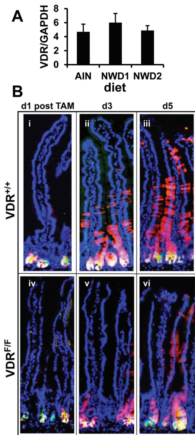
Fig. 2. The VDR in intestinal stem cell function. (A) GFP marked cells were isolated by FACS from single cell suspensions of purified intestinal crypts of Lgr5 GFP+ mice fed AIN76A, NWD1 or NWD2 diet from weaning for 6 months. mRNA levels for VDR and for GAPDH were determined by quantitative real-time PCR for the Lgr5 GFP+ cells of three mice in each dietary group (mean ± std) with each sample assayed in quadruplicate; (B) Lgr5 GFP+ , Rosa26 RFP+ , VDR flx/flx or +/- mice, nine mice per group were fed AIN76A diet for 3 months, given a single tamoxifen injection and three mice of each group killed 1, 3 or 5 days thereafter. Frozen sections of the intestine were stained with DAPI.
