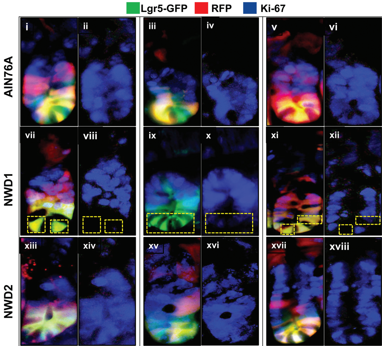
Fig. 4. Ki67 positive cells at the crypt base in mice fed different diets. Lgr5 GFP+ , Rosa26 RFP+ mice were from the experiment shown in Figure 1B : mice were fed AIN76A, NWD1 or NWD2 diets from weaning, given a single injection of tamoxifen at 3 months and then killed 3 days later, three mice per dietary group. Frozen sections of the intestine were stained with antibody to Ki67 (rabbit anti-mouse, Novus Biologicals, 1:200) detected with a secondary goat anti-rabbit Ab conjugated to Alexa Fluor 350 (Invitrogen, 1:200). The crypts were photographed separately for green, red and blue emission, representing the GFP and RFP expressed in Lgr5+ cells and their progeny, and the expression of Ki67, respectively. Images at the three different wavelengths for each crypt shown were overlaid; shown next to each of these crypts is the isolated blue fluorescence, indicating expression of Ki67.
