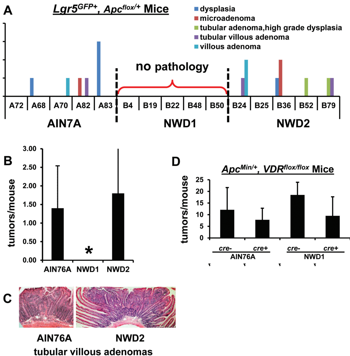
Fig. 3. Effect of diet or vitamin D receptor inactivation on Apc initiated tumor development. (A–C) Lgr5 GFP+ , Apc flox/+ mice, five mice per dietary group were fed diets from weaning for 3 months, received a single injection of tamoxifen and then continued on their respective diets for 6 more months before killing and evaluation of histopathology. (A) tumor incidence and histopathology for each of the five mice in each dietary group; (B) mean tumor incidence per dietary group \pm std (* P < 0.03, analysis of variance); (C) examples of histopathology of tumors from mice fed AIN76A or NWD2; (D) Apc Min/+ , VDR flox/flox mice that were cre(-) or villin-cre+ were fed AIN76A or NWD1 for 4 months, killed, sections from formalin fixed swiss rolls of the small intestine were stained with hematoxylin/eosin and tumor multiplicity determined.
