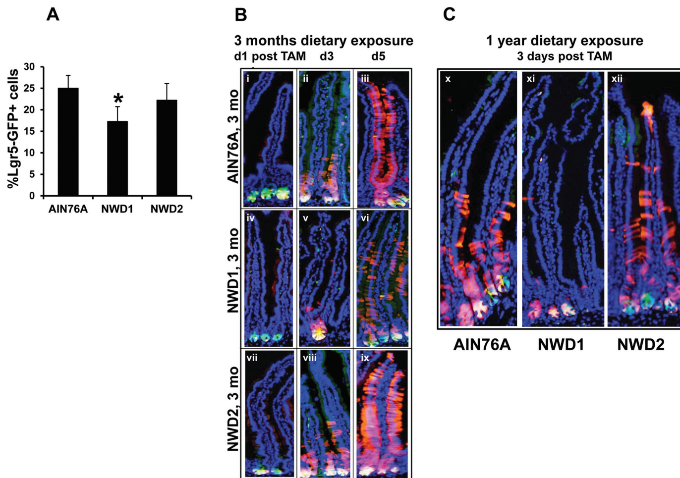
Fig. 1. Dietary effects on Lgr5 GFP+ cells in the small intestine. (A) Lgr5 GFP+ mice, four per dietary group were fed AIN76A, NWD1 or NWD2 diets from weaning for 3 months. Single suspensions of epithelial cells were prepared from isolated intestinal crypts and percent of these cells exhibiting green fluorescence determined by FACS analysis (mean \pm std; * P < 0.03, analysis of variance); (B) Lgr5 GFP+ , Rosa26 RFP+ mice, nine per dietary group were fed diets from weaning for 3 months, then given a single injection of tamoxifen and three mice in each group killed at 1, 3 or 5 days later; (C) Lgr5 GFP+ , Rosa26 RFP+ mice were fed diets from weaning for 1 year, then given a single injection of tamoxifen and killed 3 days later. In (B) and (C), frozen sections of the intestine were stained with DAPI.
