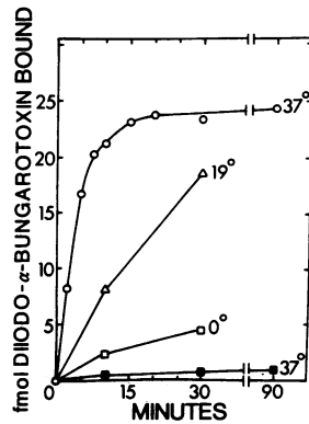
FIG. 1. The rate of ^{125}\text{I} - \alpha BT binding. Portions of a 2-week-old chick retina homogenate (62.2 \mu\text{g} of protein per reaction mixture) were incubated with 1 nM ^{125}\text{I} - \alpha BT with or without 2 \mu\text{M} unlabeled \alpha BT at the temperatures and times specified.
