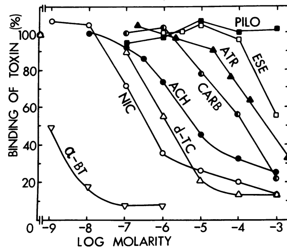
FIG. 3. Inhibitors of ^{125}\text{I} - \alpha BT binding. Portions of a 2-week-old chick retina homogenate (50 \mu\text{g} of protein per 80 \mu\text{l} of reaction mixture) were incubated for 5 min at 20° in the presence of the compounds indicated. ^{125}\text{I} - \alpha BT (10 nM) then was added (the final volume was 100 \mu\text{l} ) and tubes were incubated for an additional 10 min at 20°. The final concentration of each compound is indicated on the abscissa. Tubes with acetylcholine also contained 3 \mu\text{M} eserine sulfate. One hundred percent on the ordinate corresponds to 6.25 fmol of ^{125}\text{I} - \alpha BT specifically bound in the absence of inhibitor. This value was 35% of that obtained after 30 min of incubation at 37°. Abbreviations represent the following: \alpha -BT, unlabeled \alpha -bungarotoxin; NIC, nicotine; d-TC, d -tubocurarine; ACH, acetylcholine plus 3 \mu\text{M} eserine sulfate; CARB, carbamylcholine; ATR, atropine; ESE, eserine sulfate; PILO, pilocarpine.
