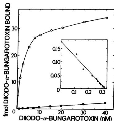
FIG. 2. Relation between ^{125}\text{I} -diiido- \alpha BT concentration and the amount of labeled toxin bound. Portions of a 2-week-old chick retina homogenate (62.2 \mu\text{g} of protein per reaction mixture) were incubated for 5 min at 20°, in the absence (O), or presence (●), of 2 \mu\text{M} unlabeled \alpha BT. ^{125}\text{I} -Labeled \alpha -bungarotoxin then was added at the concentrations specified and the reaction mixtures were incubated and assayed for bound radioactivity as described in Materials and Methods . A Scatchard plot of specific ^{125}\text{I} - \alpha BT binding; i.e., binding obtained after subtracting the radioactivity bound in the presence of 2 \mu\text{M} unlabeled toxin, is shown in the insert; the ordinate refers to the bound/free ^{125}\text{I} - \alpha BT ratio; the abscissa corresponds to nM toxin bound per 62.2 \mu\text{g} of protein.
