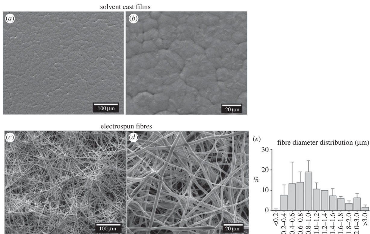
Figure 1. Scanning electron microscopy (SEM) photomicrographs of the prepared P(TMC-CL) surfaces. (a,b) Films obtained by solvent casting and (c,d) fibres obtained by electrospinning. (e) Fibre diameter distribution as calculated from 100 measurements from three independent samples (average \pm s.d.).
