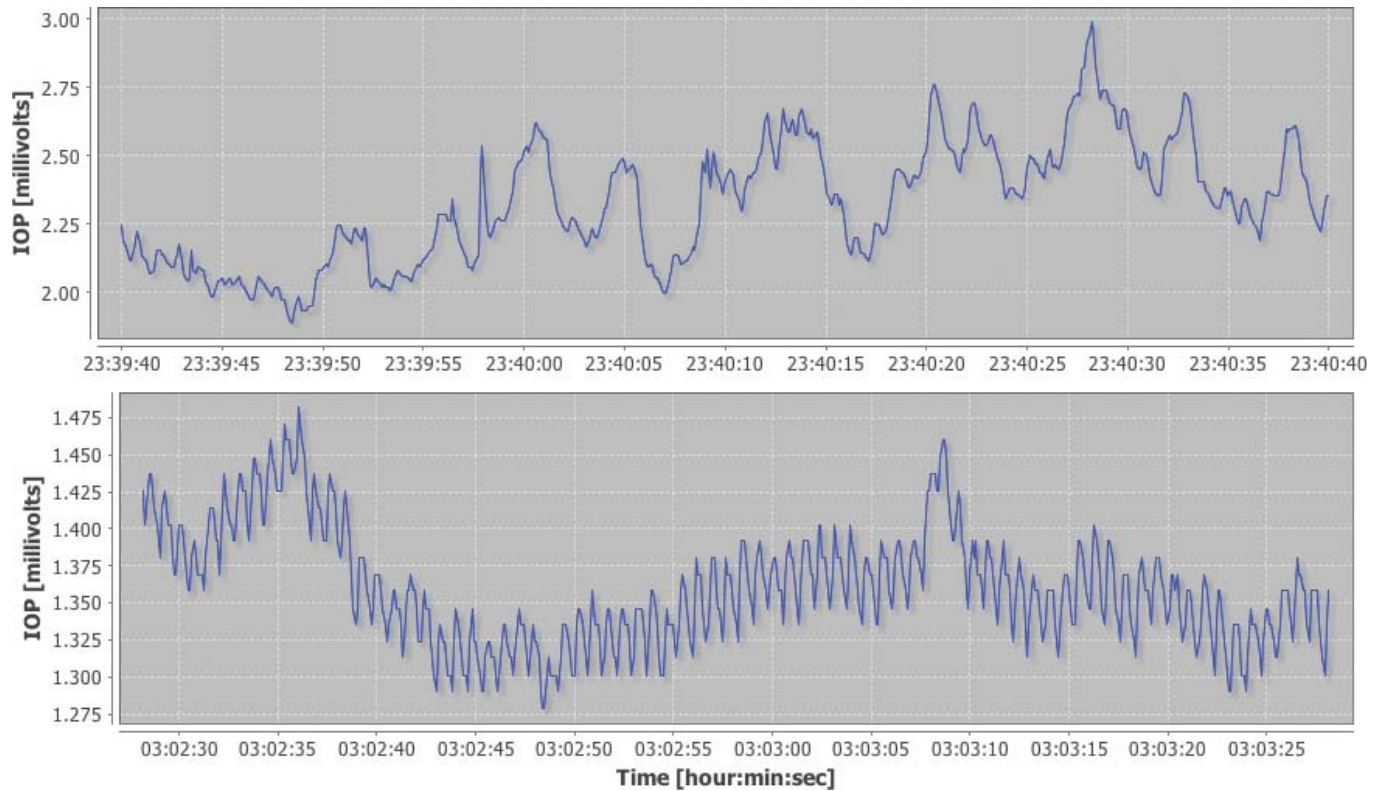
Figure 4. Examples of bursts captured during a sleep period, that is while a patient was asleep (early sleep, top and late sleep, bottom ). The absence of blinks ensures that the monitored patient was asleep at that time (confirmed with subject diary). Differences in patterns correspond to different sleep stages.
