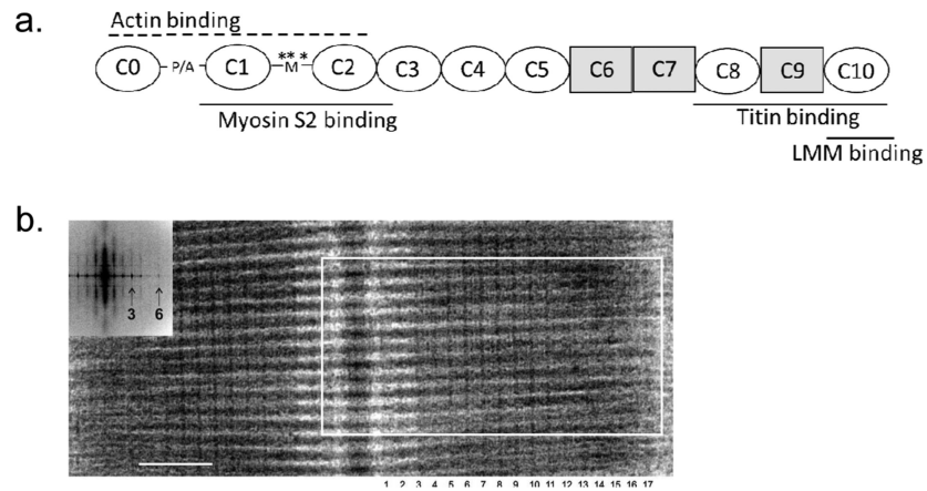
Fig. 1. a Schematic representation of myosin binding protein C (MyBP-C). Shown are Ig-like domains (ovals) and Fn-III like domains (rectangles). The cardiac isoform of MyBP-C has an extra domain at the N-terminus (C0) and additional phosphorylation sites in the M-domain between C1 and C2 (asterisks) b Electron micrograph image demonstrating the stripes where MyBP-C is located. Pictures from Luther et al. [52]
