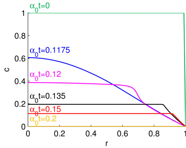
(a) Scheme 1
