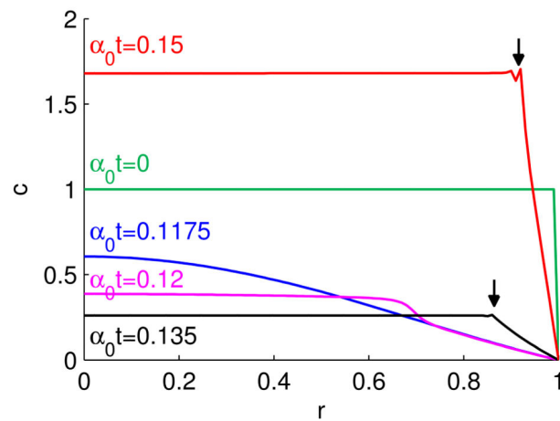
(b) Scheme 2
