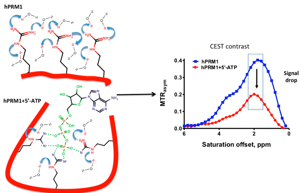
Figure 3. Cartoon of CEST contrast of hPRM1 alone (upper) and complexed with 5'-ATP (lower), which resulted in a decrease of CEST contrast in MTR_{asym} . B_1 = 3.6 \mu\text{T} , T_{sat} = 4 \text{ s} .
