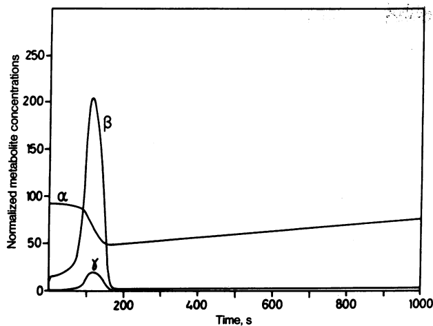
FIG. 4. Relay of a cAMP signal. The situation is that shown in Fig. 2 except that ATP injection rate v is decreased by a factor of 2.5. Initially, intracellular ATP ( \alpha ) and intracellular cAMP ( \beta ) have their steady-state values. Exterior stimulation is simulated by setting extracellular cAMP at a value that is two times its steady-state level (the steady-state values are \alpha = 92.366 , \beta = 10 , and \gamma = 1 ).
