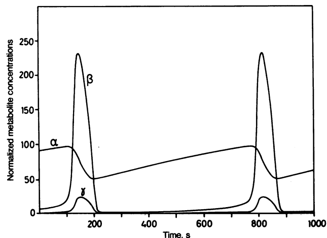
FIG. 2. Autonomous periodic oscillations of normalized concentrations of intracellular ATP ( \alpha ), intracellular cAMP ( \beta ), and extracellular cAMP ( \gamma ). The curves are obtained by integration of Eqs. 2, for v = 0.1 \text{ s}^{-1} ; other parameter values are given in the legend to Table 1.
