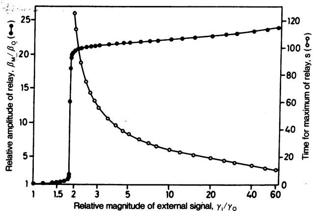
FIG. 5. Dependence of the relay response on the amplitude of the external cAMP signal. The curves give the amplitude and the time course of relay as a function of the ratio ( \gamma_i/\gamma_0 ), where \gamma_i and \gamma_0 are the initial and steady-state values of the normalized concentration of external cAMP (in the case considered, \gamma_0 = 1 ), respectively. The amplitude of relay is given as the maximum of the intracellular cAMP peak, \beta_M , divided by the steady-state level \beta_0 . The second curve shows the time at which the maximum of the peak, \beta_M , is reached after the initial stimulation. Parameter values are those of Fig. 4.
