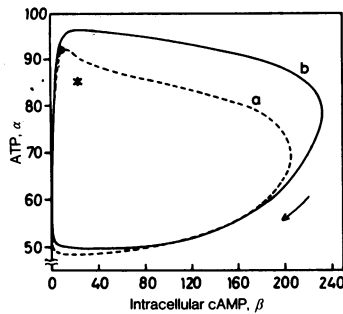
FIG. 6. A trajectory for relay and for oscillation in the (\alpha, \beta) phase plane. In curve a, relay starts at the steady-state values of \alpha and \beta (●), following a slight increase in the third variable \gamma . Curve b shows a limit cycle enclosing the unstable steady state (*). The arrow indicates the direction of movement. The situations described by curves a and b are those of Figs. 4 and 2, respectively.
