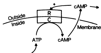
FIG. 1. Compartmental model for relay and oscillation of cAMP. Capitals R and C refer to the receptor and to adenylate cyclase, respectively. The + sign indicates that binding of cAMP to the receptor results in cyclase activation (see details in text ).
