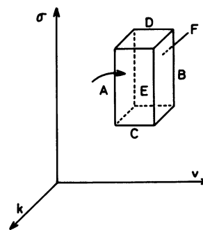
FIG. 3. The rectangular parallelepiped schematizes a domain in which autonomous oscillations can be found in a parameter space composed of ATP injection rate ( v ), adenylate cyclase activity ( \sigma ), and phosphodiesterase activity ( k ). The letters A through F represent regions exterior to the six faces of the parallelepiped in which relay capability was sought. The heavy arrow entering the parallelepiped through A represents a slow developmentally controlled parameter variation that could bring about the observed transitions between cells whose cAMP production is always small (inert cells), amplifies cAMP signals (relay cells), or spontaneously and periodically reaches significant levels (autonomous oscillators).
