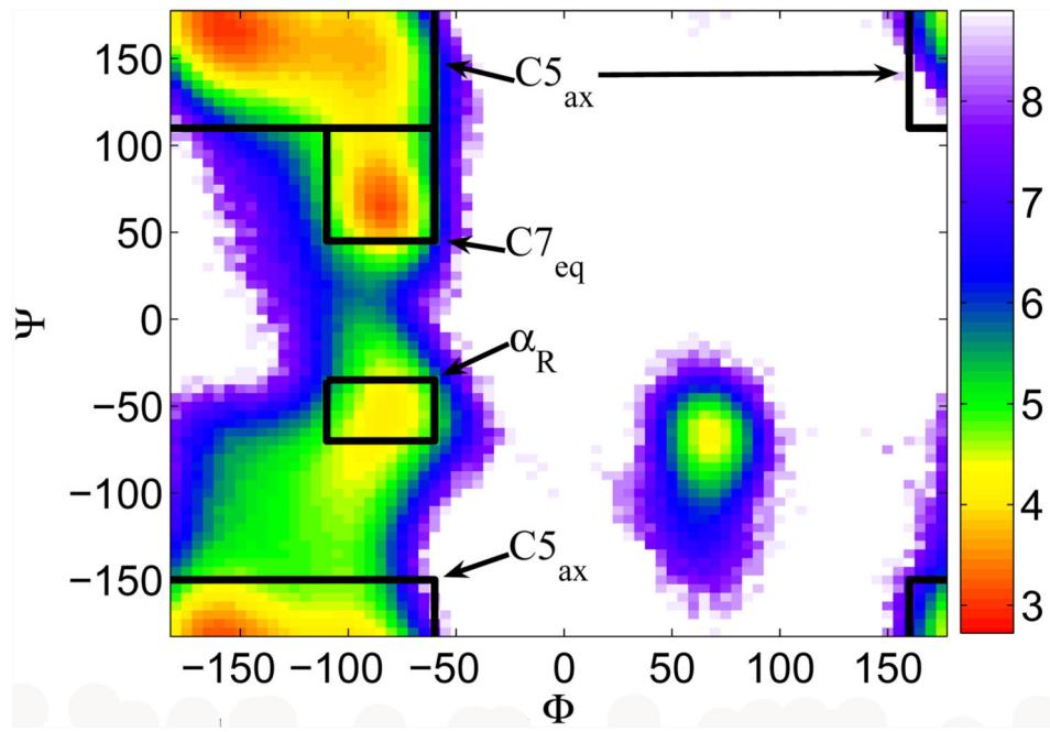
Fig. 6. Free energy for alanine dipeptide
