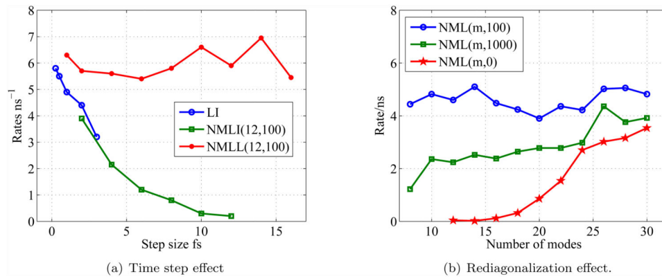
Fig. 7. Isomerization rate as (a) function of time step for different Langevin integrators, and (b) different rediagonalization periods. Error bars are smaller than the symbol sizes.
