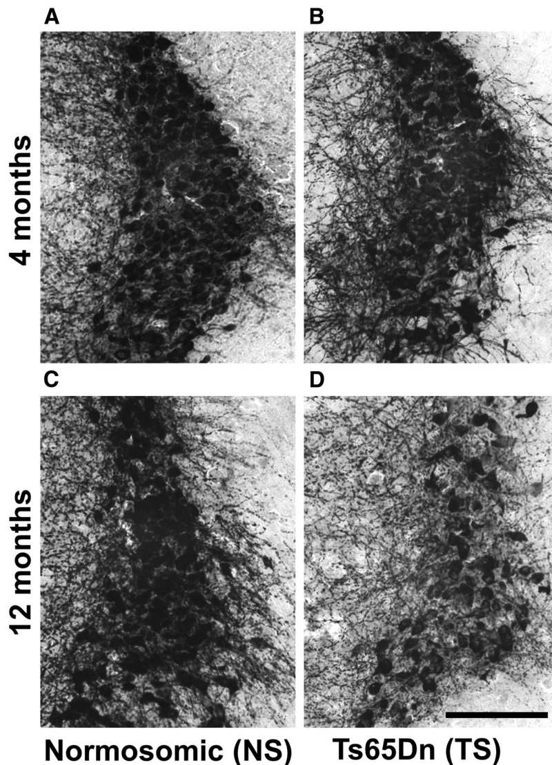
Figure 1. TH immunostaining in the LC-NE region of Ts65Dn mice and NS mice at 4 and 12 months of age. A, B, At 4 months of age, there was no difference in terms of TH staining density between NS ( A ) and Ts65Dn ( B ) mice. C, D, However, at 12 months of age, there was a marked reduction in TH-immunoreactive fiber density and cell-packing density in Ts65Dn mice ( D ), compared with NS mice ( C ). TH-positive LC cell bodies had observable degenerative morphology, including a pyknotic nucleus and reduced intracellular TH staining in Ts65Dn mice ( D ). Representative images taken at 10 \times magnification. Scale bar, 200 \mu m.
