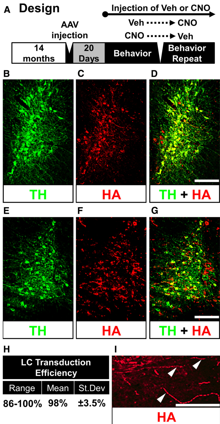
Figure 2. TH and HA immunostaining in the LC. A , Experimental design for the DREADD study. The AAV-HA tag vector was injected via stereotaxic injections into Ts65Dn or NS mice. Twenty days after surgery, mice were tested for behavior. After a 2 d washout period, mice were given the opposite treatment in a crossover design. B–D , TH immunostaining ( B , green), HA staining ( C , red), and overlay ( D , yellow) in a normosomic mouse LC. E–G , TH ( E , green), HA ( F , red), and overlay ( G , yellow) in the LC of a Ts65Dn mouse. H , Transduction efficiency table, showing range, mean, and SD measured in a total of 19 double-labeled sections. I , FITC-labeled HA immunostaining in the LC region at a higher magnification, with evidence of axonal transport of the DREADD receptors (arrowheads). Scale bars: D, G , 100 \mu m; I , 40 \mu m.
