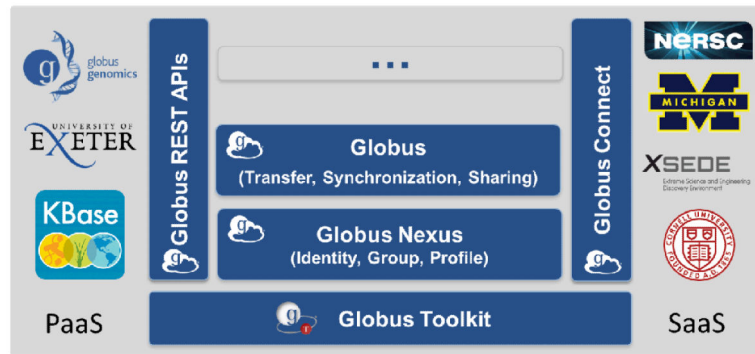
Figure 1. Globus services provide users with research data management functions (right) but also implement REST APIs that permit their use as a platform (left).
