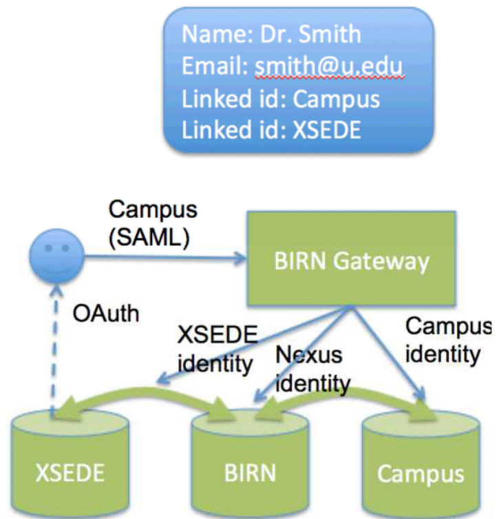
Figure 5. Globus Nexus identity hub example, showing use of multiple identities for different purposes.
