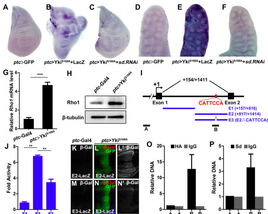
Fig. 5. Yki-Sd directly induces Rho1 transcription. (A–F) Knocking down sd suppresses Yki-induced Rho1 transcription. In situ hybridization to Rho1 mRNA of third instar wing discs (A–C) or salivary gland (D–F) expressing GFP (A and D), Yki S168A + LacZ (B and E), Yki S168A + sd RNAi (C and F) driven by ptc -Gal4. (G and H) Ectopic Yki up-regulates Rho1 mRNA (G) and protein (H) levels, as shown by quantitative PCR and Western blot, respectively. ( n = 200, mean + SD, *** P < 0.001) (I) Scheme of the Rho1 locus showing the first intron. The Sd binding motif (CATTCCA) is indicated. E1, E2, and E3 were used to drive luciferase expression; A and B represent the control and target region of ChIP assays, respectively. (J) Luciferase assay in Drosophila S2 cells. ( n = 3, mean + SD, ** P < 0.01) (K–N) The Sd binding motif is required for Yki-induced target gene expression in vivo. Compared with the controls (K and M), ectopic expression of Yki S168A along the A–P compartment boundary results in dramatic up-regulation of E2-LacZ (L), but not E3-LacZ (N). (O and P) Drosophila S2 cells transfected with Sd and Yki-HA were used for quantification of ChIP-PCRs. ( n = 3, mean + SD).
