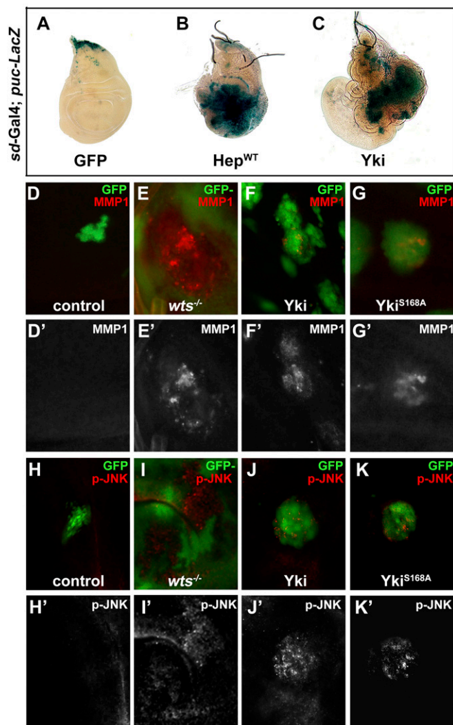
Fig. 1. Yki activates JNK signaling in Drosophila . Third instar wing discs are shown. Ectopic Yki activates JNK target puc expression. puc-LacZ expression is shown in sd > GFP control (A), sd > Hep WT (B), and sd > Yki (C) wing discs. Compared with control clones (D and H), impaired Hippo signaling activates MMP1 expression and JNK phosphorylation in wts mutant clones (E and I), or clones expressing Yki (F and J) or Yki S168A (G and K). Clones were labeled by the presence (D, F, G, H, J, and K) or absence (E and I) of GFP expression. See also Figs. S1 and S2.
