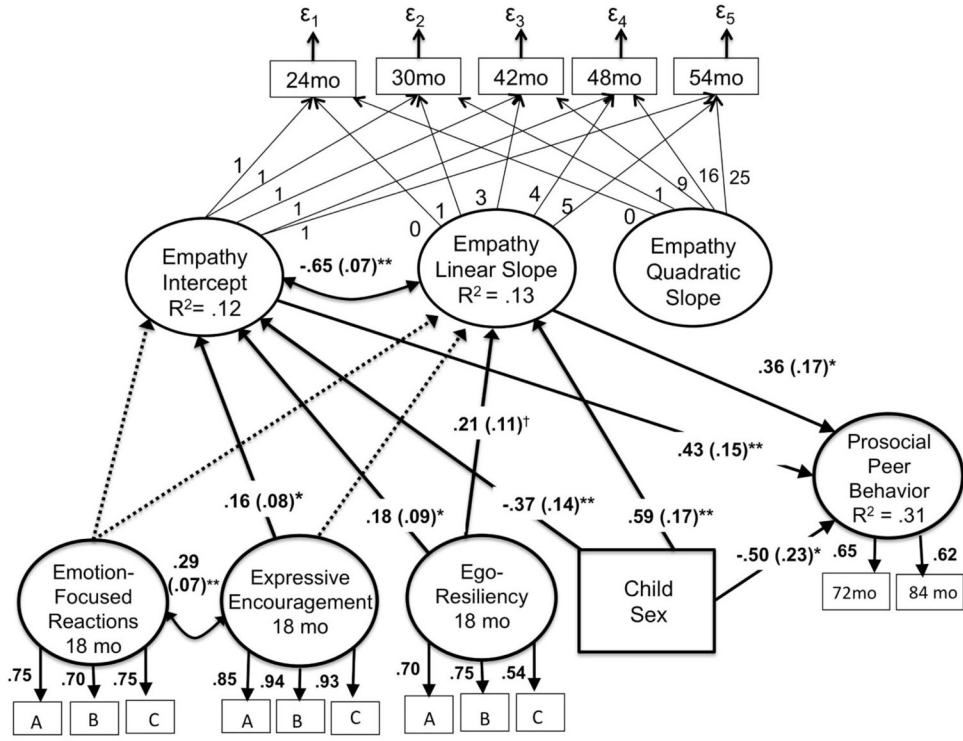
Figure 1. Results from the structural equation model. Note: \chi^2(141, N = 242) = 159.09, p > .05 ; CFI = .987; TLI = .983; RMSEA = .023; SRMR = .052. ** p < .01 , * p < .05 , † p < .10 . Factor loadings for the latent variables are all significant at p < .01 . Standardized (stdyx) coefficients are presented with the exception of paths from child sex (stdy). Ego-resiliency = combined mother and nonparental caregiver reports; Emotion-Focused Reactions (EFR, CTNES) = mother report; Expressive Encouragement, (EE, CTNES) = mother report; Empathy = mother report; Prosocial Peer Behavior = teacher report. Dotted lines are nonsignificant paths. The variance of the quadratic slope was fixed at zero, as there was no variability; therefore, predictor variables were not included. Nonsignificant paths (not shown in the model for simplicity, but included in the analyses) were ego-resiliency with EFR, EE, and child sex; child sex with EFR and EE; ego-resiliency, EFR, and EE to prosocial behavior. The path from ego-resiliency to the slope of empathy was marginally significant ( p = .054 ).
