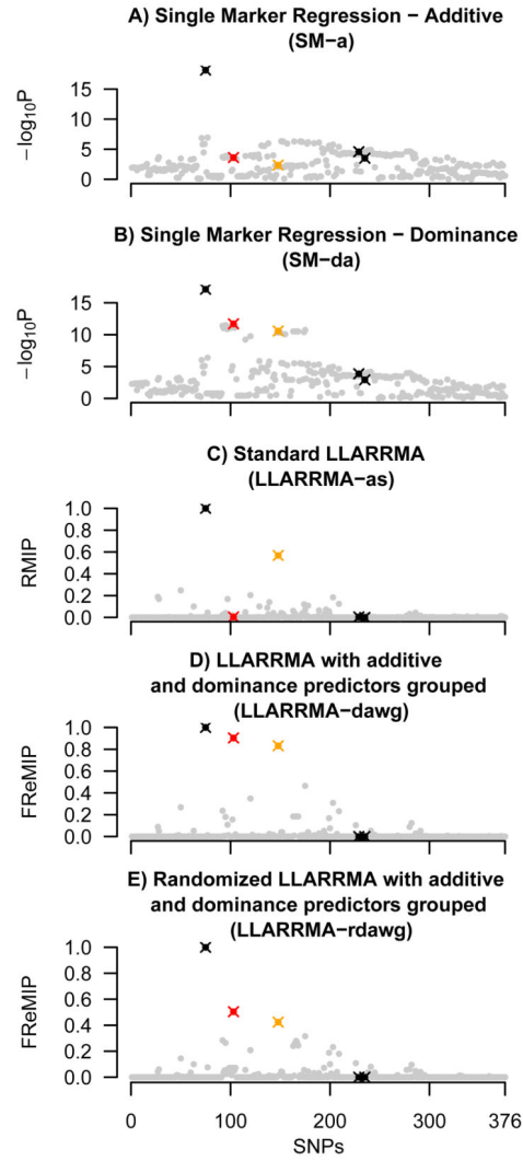
Figure 2. Results of five methods applied to an example dataset from simulation study G. Plots show SNP location in a simulated locus against SNP score, where SNP score is defined for single marker methods (sub plots A, B) as -\log_{10} of the p-value ( \log P ), and for multi-SNP methods as the inclusion probability (RMIP or FReMIP). SNPs for which a true signal was simulated are shown as crosses, in black (additive effect), orange (major allele dominant), and red (minor allele dominant); all other (background) SNPs are shown gray dots.
