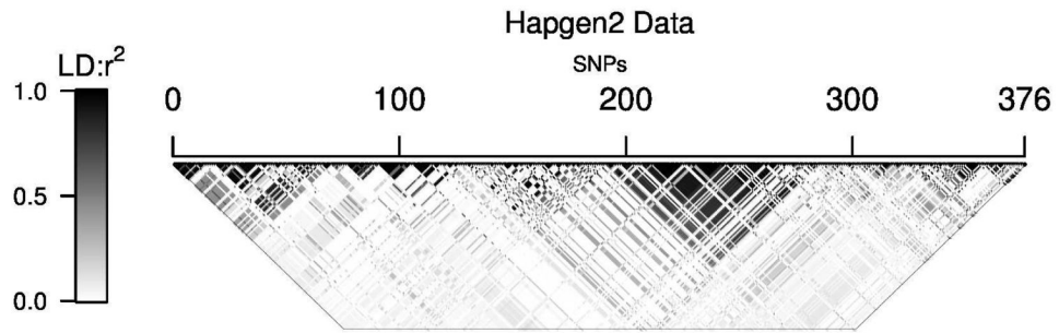
Figure 1. LD structure used by HAPGEN2 to create simulated genotype data. Shading indicates pairwise LD between SNPs, ranging from white ( r^2 = 0 ) to black ( r^2 = 1 ).
