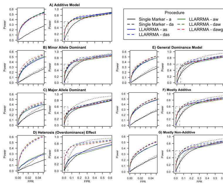
Figure 3. Initial and full ROC curves plotting discriminatory power of single marker and multi-SNP (LLARRMA) methods under seven simulation settings. Each setting (A–G) corresponds to the presence of a different underlying genetic architecture for the locus, and plots both the full ROC curve (right) and its zoom-in (the initial ROC; left); better performance in each case is indicated by a greater area under the initial ROC curve. For clarity, only multi-SNP methods using constant penalization are shown.
