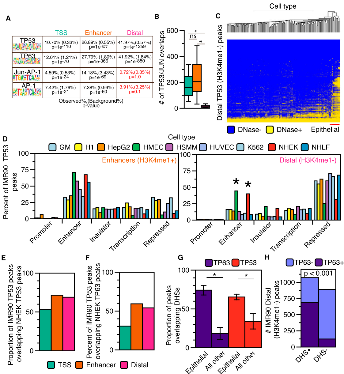
Figure 5. Distal (H3K4me1-) TP53 peaks bind to accessible chromatin in a cell-specific manner. (A) Transcription factor motif analysis for enhancer and distal TP53 peaks using HOMER. (B) Boxplot of JUN/FOS/TP53 colocalization at the three categories of TP53 binding sites. Asterisks denote that the P -value for the pairwise comparison is less than 0.05 (Wilcoxon rank sum test). (C) Hierarchical clustering (Euclidean distance) of the overlap between TP53 distal (H3K4me1-) peaks and DHSs from the ENCODE Project (minimum of 1-bp overlap between TP53 and DHSs; additional information in Supplemental Table S5). (D) Analysis of the overlap between TP53 enhancer (orange) and distal (pink) peaks with ChromHMM-defined genomic regulatory regions from nine human cell types. Similar functional ChromHMM categories were grouped into single categories (i.e., strong and weak enhancers grouped together). TP53 peaks were allowed to overlap multiple ChromHMM regulatory regions, and each region was reported (minimum of 1-bp overlap). (E) The proportion of IMR90 TP53 peaks overlapping TP53 binding sites from cisplatin-treated normal human epithelial keratinocytes (NHEK). (F) The proportion of IMR90 TP53 peaks overlapping TP63 binding sites from cisplatin-treated NHEK. (G) The proportion of TP63 (NHEK) and TP53 (IMR90) binding sites overlapping regions of DHSs from epithelial cell types and all other cell types with available data. P -values generated using a two-tailed t -test ( P -values < 0.001). (H) Dependency of TP53 distal (H3K4me1-) peak overlap with DHSs (normal human epithelial keratinocytes) on co-occupancy with TP63: P -value < 0.001 ( \chi^2 test).
