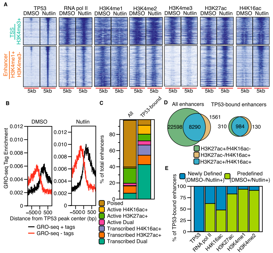
Figure 3. TP53 binds to established H3K4me1-marked enhancers and recruits RNA pol II and H4K16ac. (A) Heatmaps of TP53, RNA pol II, H3K4me3, H3K4me1, H3K27ac, and H4K16ac enrichment within a 5000-bp window ( \pm 2500 bp from the TP53 peak center) for TSS (H3K4me3+) and enhancer (H3K4me1+/H3K4me3-) TP53 peak types after DMSO or nutlin treatment. (B) Average GRO-seq profiles (normalized to 1 \times 10^{-7} reads) at TP53 enhancer (H3K4me1+/H3K4me3-) peaks after DMSO or nutlin treatment. (C) Distribution of combinatorial histone modifications and RNA pol II enrichment at TP53-bound H3K4me1+ enhancers compared to the genome-wide complement of H3K4me1+ enhancers. (Poised enhancers) H3K4me1+; (active enhancers) H3K4me1+ and at least one acetylation event (H3K27ac or H4K16ac); (transcribed enhancers) H3K4me1+, RNA pol II+, and at least one acetylation event (H3K27ac or H4K16ac). Dual enhancers are occupied by both H4K16ac and H3K27ac. (D) Venn diagram representation of the overlap between H3K27ac+ and H4K16ac+ enhancers for all genome-wide and TP53-bound enhancers. (E) Analysis of the preestablishment of occupancy for each indicated factor at TP53-bound enhancers. Predefined enhancers are those in which the surveyed factor was significantly enriched (MACS-defined) during the DMSO treatment (no TP53 activation), whereas newly defined enhancers are those in which the enrichment of each factor was dependent on treatment with nutlin.
