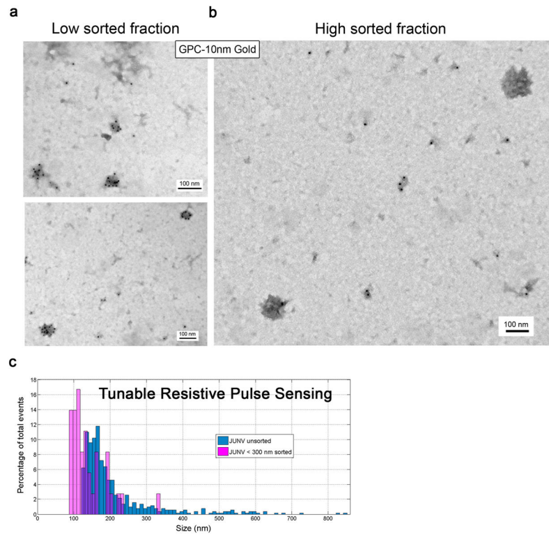
Figure 2. Sorting of infectious viruses by flow virometry. (a,b) JUNV-A647 particles were sorted directly onto carbon-coated TEM grids and labeled with the GPC specific GD01 antibody followed by a secondary antibody, then revealed by Protein A 10 nm gold beads. The low (a) and high (b) fractions were negatively staining and analyzed by transmission electron microscopy. Several particles per micrograph are shown and the images are representative of each population. The low fraction viruses are about 60 nm in diameter, while the high fraction viruses are around 150 nm. (c) Tunable Resistive Pulse Sensing (TRPS) was performed on unsorted (blue bars) or sorted particles smaller than 300 nm (pink bars). The histograms show the distribution of particle size detected in each sample.
