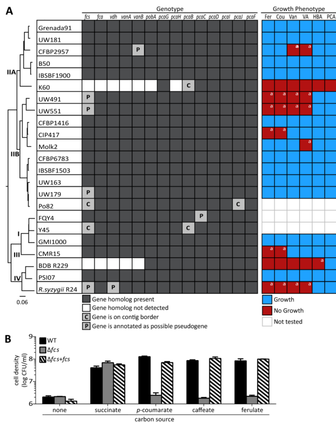
Fig. 2. HCA degradation is widely conserved in the R. solanacearum species complex. A , Genetic and functional conservation of HCA degradation. A whole genome comparison phylogenetic tree is shown on the left. Presence of HCA degradation genes and growth of R. solanacearum strains on ferulate (Fer), p -coumarate (Cou), vanillin (Van), vanillate (VA), p -hydroxybenzoate (HBA), and protocatechuate (PCA) are indicated. a Growth phenotype differs from genotype prediction; B , fcs encodes a functional feruloyl-CoA synthetase in strain GMI1000. Strains were grown in minimal media supplemented with 0.2 mM succinate, p -coumarate, caffeate, ferulate, or no carbon (–) for 72 hr. Bars represent the mean of 3 biological replicates and error bars indicate standard error of the mean.
