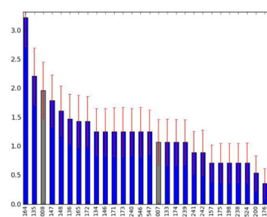
(c) EF 10%
