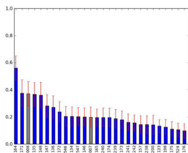
(a) BEDROC
