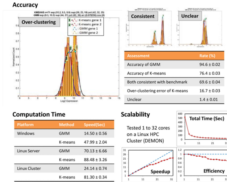
Fig. 3. Performance of the GMM peak calling pipeline comparing with the original LINCSeq pipeline.
