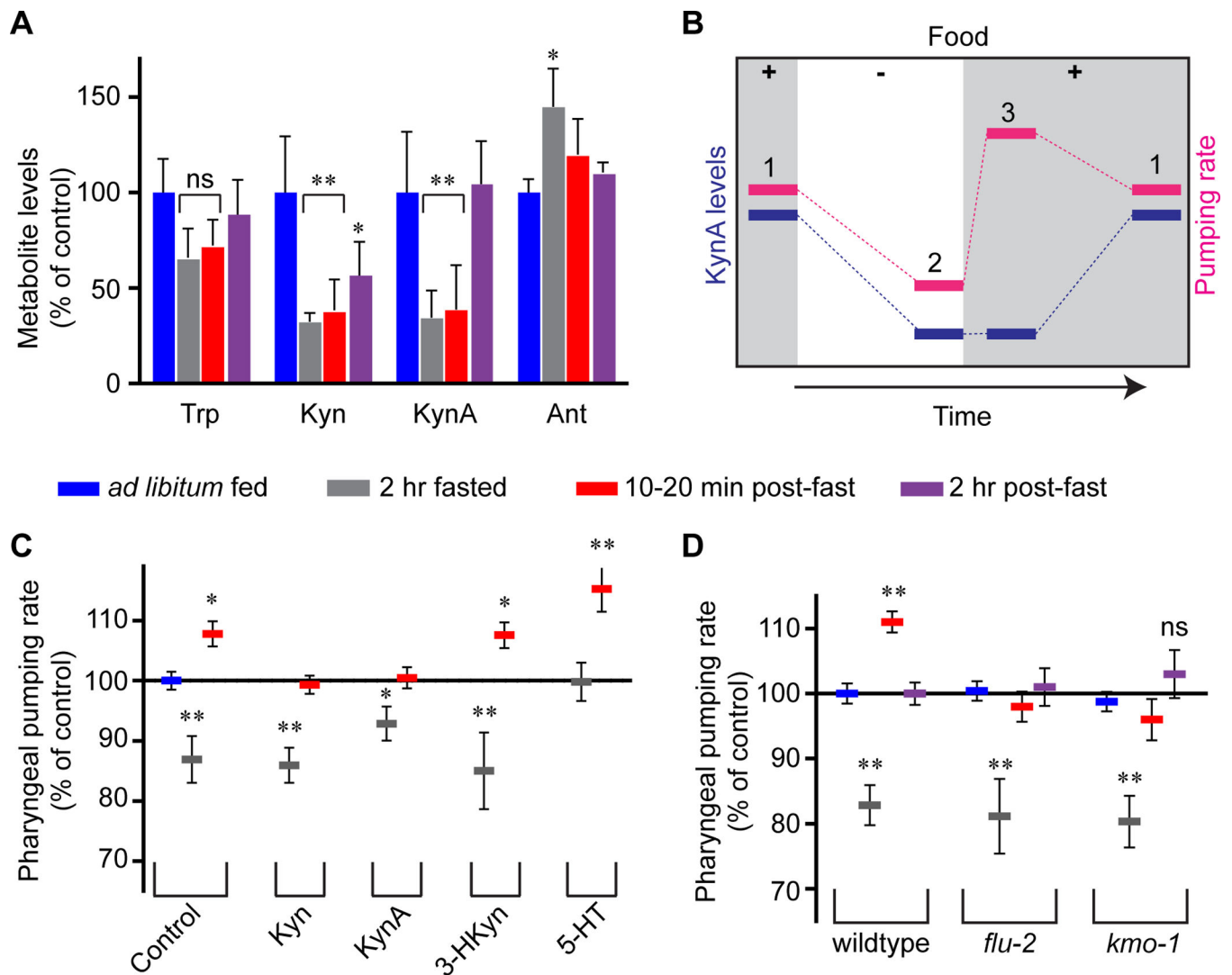
Figure 3. KynA Depletion During Fasting Is Required For Post-fast Hyperactive Feeding (A) Determination of tryptophan (Trp), kynurenine (Kyn), kynurenic acid (KynA) and anthranilic acid (Ant) from extracts of wildtype C. elegans fed ad libitum , after 2 hr of fasting, after 20 min or 2 hr of post-fast feeding. For each metabolite, data are normalized to the ad libitum fed condition. Error bars = s.d. of 3–4 independent cultures ns: p > 0.05 , * p < 0.05 , ** p < 0.0001 ANOVA (Tukey) relative to ad libitum fed for each metabolite. (B) Observed relationships between KynA levels, pharyngeal pumping rate, and food availability with time indicating three distinct behavioral states (1–3). (C) Effects of metabolite supplementations on pharyngeal pumping rates of wildtype C. elegans . During the fasting period animals were treated with either vehicle, or 100 \mu\text{M} of each of Kyn, KynA, 3-hydroxykynurenine (3-HKyn) and serotonin (5-HT). n=10-12 animals per condition. ns p > 0.5 , * p < 0.01 , ** p < 0.0001 ANOVA (Holm-Sidak) compared to ad libitum fed control. (D) Pumping rates from wildtype and mutants at the indicated fasting and refeeding periods. n = 12-14 animals per condition. ns: p > 0.05 , ** p < 0.0001
