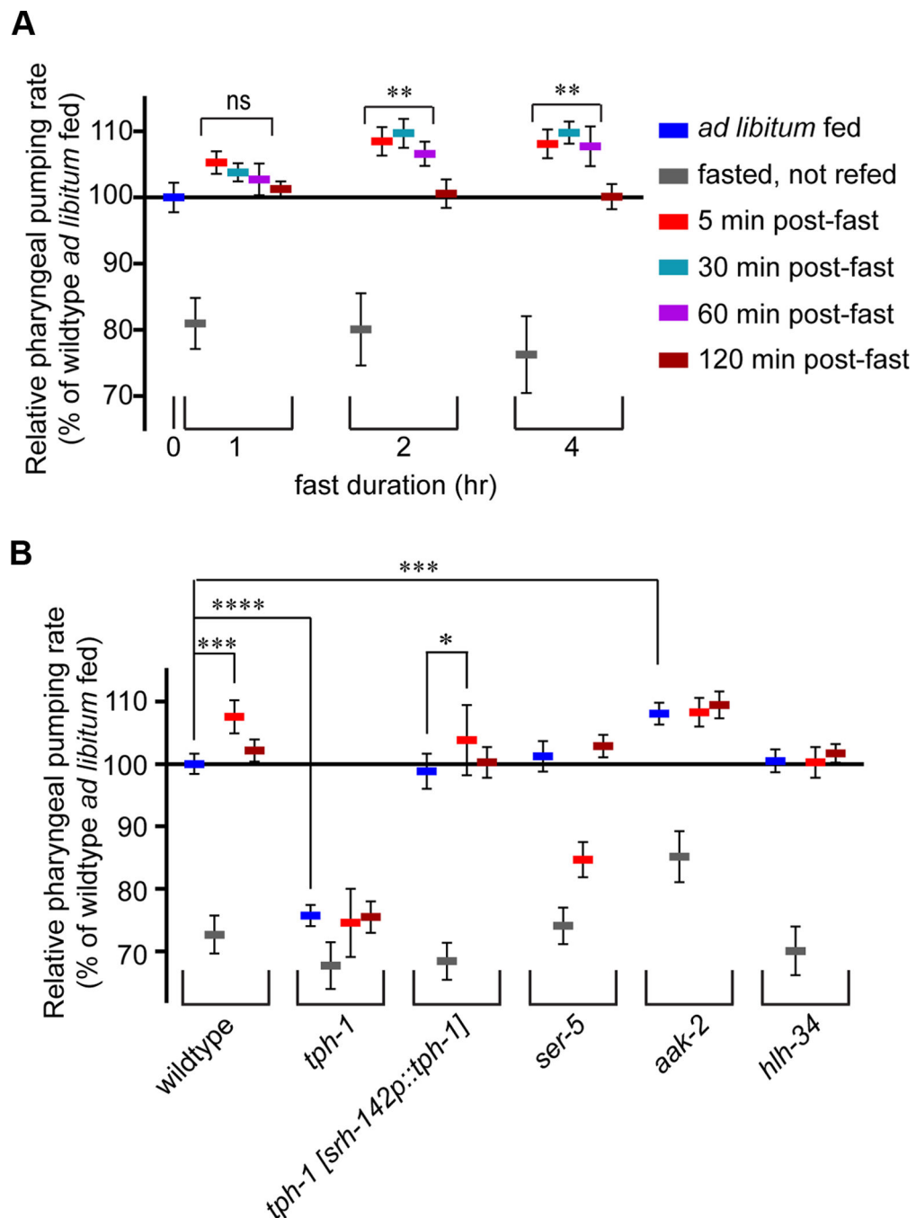
Figure 1. Post-fast Hyperactive Feeding Requires Serotonin Signaling
