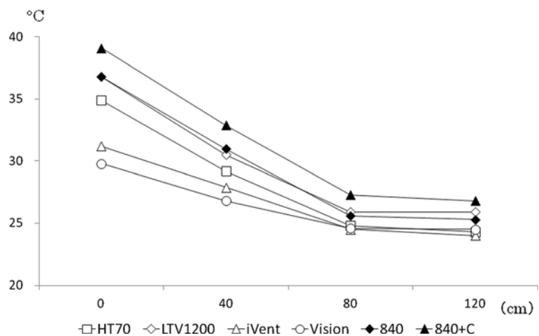
Figure 3 Effect of distance from outlet on temperature of gas delivered from the ventilators. For each ventilator, by the time the gas had traveled 40 cm from the outlet, gas temperature fell less than 35^{\circ}\text{C} .
