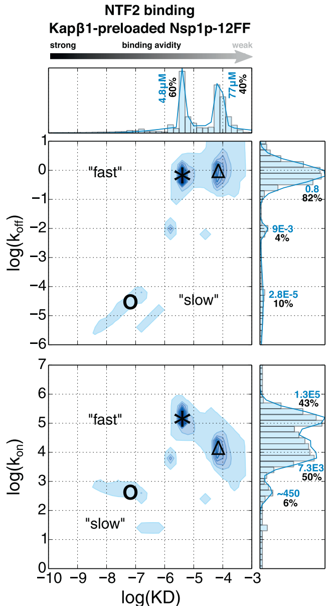
FIGURE 6 Multivalent kinetic analysis of NTF2 binding close-packed Nsp1p FG domains preloaded with Kap \beta 1. Two-dimensional interaction maps of kinetic on- and off-rates ( k_{\text{on}} and k_{\text{off}} , respectively) are shown in relation to the equilibrium binding constant KD. The fractional abundance of different kinetic states is indicated by the color intensity and the sum over all values in a given axis is shown as accompanying histograms (top and right panels). Different kinetic species are labeled with O (high-affinity slow phase), * (mid-affinity fast phase), and \Delta (low-affinity fast phase). Each distribution is given in percent of the total sum and their main values are depicted in bold. Units are \text{s}^{-1} and \text{s}^{-1}\text{M}^{-1} for k_{\text{off}} and k_{\text{on}} , respectively. To see this figure in color, go online.
