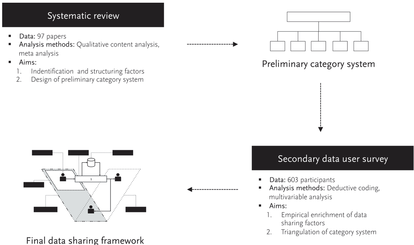
Fig 1. Research Methodology.
