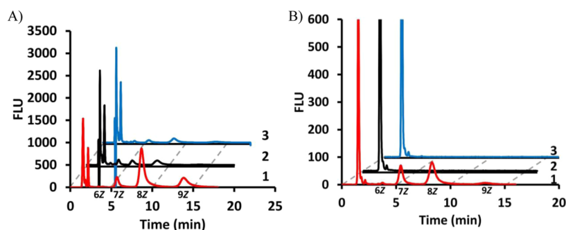
Figure 2. 2AA-GPP is an ineffective substrate for UPPS Ec and UPPS Vv . HPLC analysis of 2AA-GPP with (1, red) UPPS Bf , (2, black) UPPS Ec , and (3, blue) UPPS Vv at (A) 167 nM and (B) 1.7 \mu M. Chromatograms 2 and 3 are offset by 2 and 4 min, respectively. Note that the peaks representing flow-through material in panel B (2AA-GPP) are cut to give the best view of long chain isoprenoid products. In all chromatograms, the ESI-MS-identified product is indicated below the time axis with the number of Z-configuration isoprenes associated with each peak.
