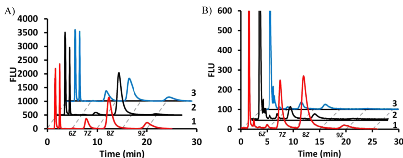
Figure 3. 2CNA-GPP is an effective substrate for all three UPPS proteins. HPLC analysis of 2CNA-GPP with (1, red) UPPS Bf , (2, black) UPPS Ec , and (3, blue) UPPS Vv at (A) 167 nM and (B) 1.7 \mu M. Chromatograms 2 and 3 are offset by 2 and 4 min, respectively. Note that the peaks representing flow-through material are cut to give the best view of long chain isoprenoid products.
