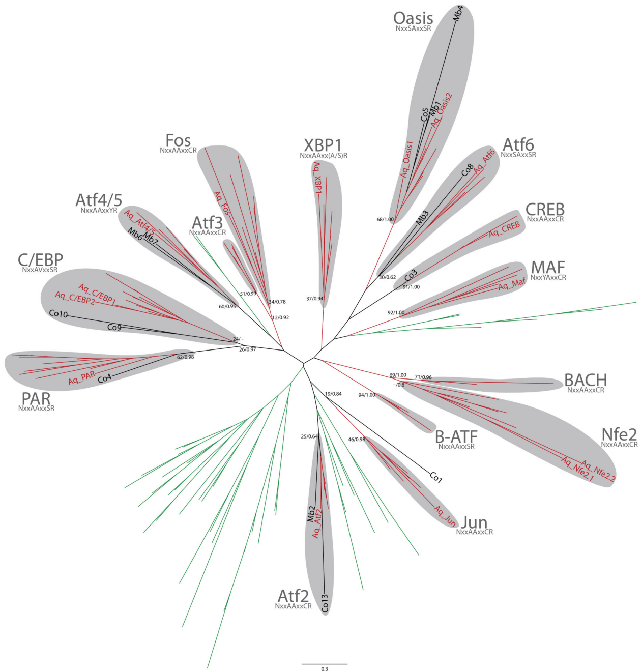
Figure 3. Maximum likelihood tree of bZIP genes including the unambiguously assigned Capsaspora bZIP homologs. The tree is rooted using the midpoint-rooted tree option. Statistical support was obtained by RAxML with 1000-bootstrap replicates (BV) and Bayesian Posterior Probabilities (BPP). Both values are shown on key branches. Aq ( A. queenslandica ), Co ( Capsaspora ), Mb ( M. brevicollis ). Metazoan branches depicted in red and fungal branches in green. For each family, the signature sequence for DNA recognition is indicated and only
