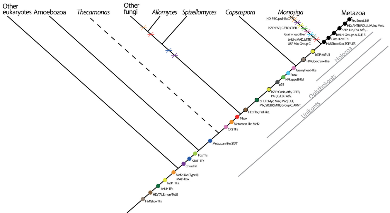
Figure 5. Cladogram representing TF evolution among the analyzed taxa. Colors are unique for each domain class. A colored dot means the hypothetical origin of the domain. A black circled dot indicates where a specific protein family appears in our taxon sampling. A cross means the loss of the domain or specific protein family in a lineage. Metazoan apomorphies are shown as black dots. The phylogenetic relationships are based on several recent studies (Burki et al. 2008; Ruiz-Trillo et al. 2008; Brown, Spiegel and Silberman 2009; Liu et al. 2009; Minge et al. 2009).
