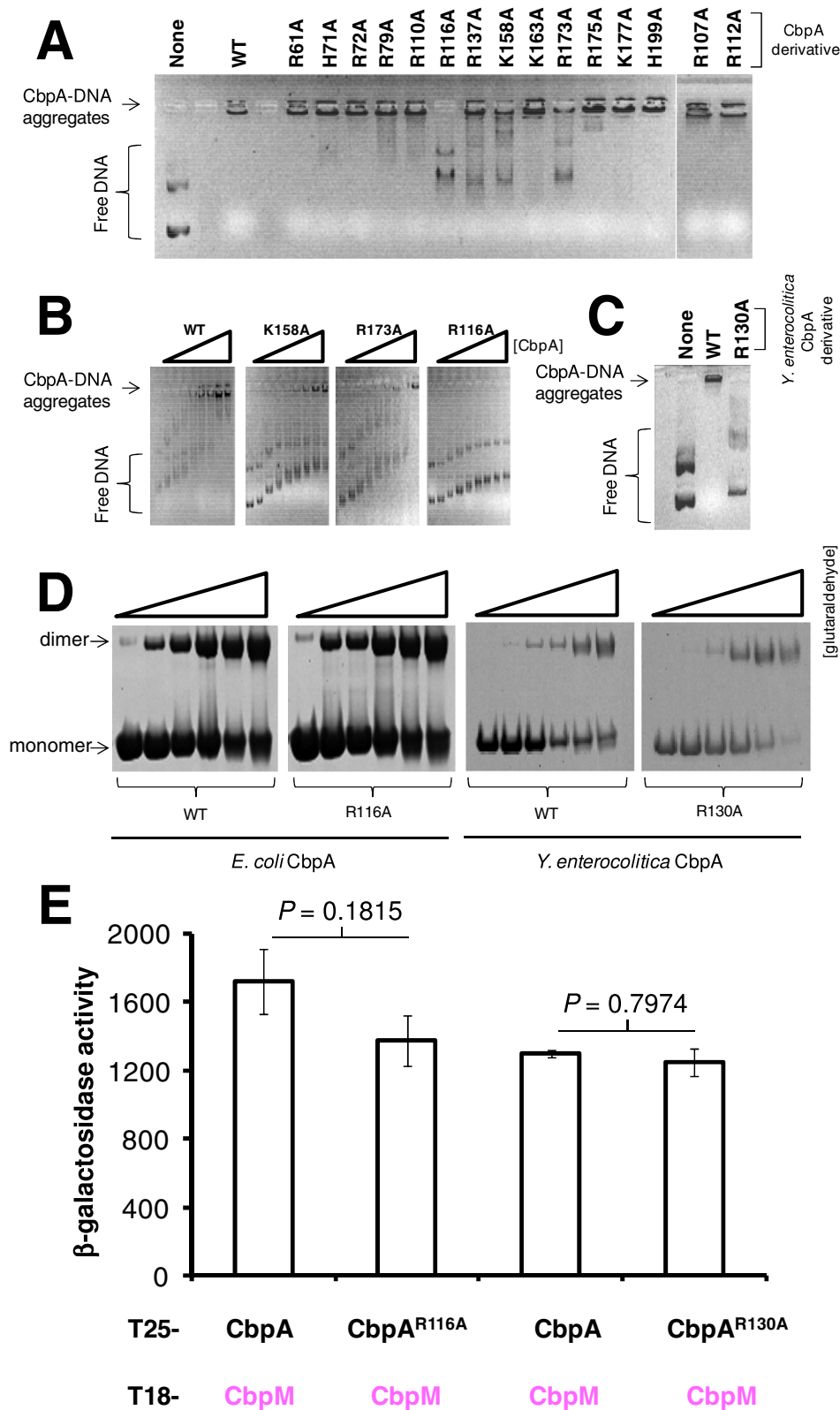
Figure 4. CbpA side chain R116 is a conserved DNA binding determinant. Panel (A) shows two 1% ( w/v ) agarose gels on which the binding of different CbpA (4 \mu M) derivatives to plasmid DNA (250 ng per lane) was analysed. Panel (B) shows DNA-aggregate formation by wild-type CbpA (and the R116A, K158A and R173A derivatives) in a set of titrations. Panel (C) is a gel shift experiment comparing binding Yersinia enterocolitica CbpA (4 \mu M) and the R130A derivative, to plasmid DNA (250 ng per lane). Panel (D) shows purified CbpA derivatives analysed on a sodium dodecylsulphate-polyacrylamide gel. Proteins (5 ng) were treated with between 0.0001% and 0.002% glutaraldehyde before loading. Monomeric and dimeric forms of CbpA are indicated. Panel (E) shows a bar chart depicting results of BACTH assays performed to measure CbpA–CbpM interactions. Different CbpA derivatives are indicated. The Student's t -test was used to calculate P .
