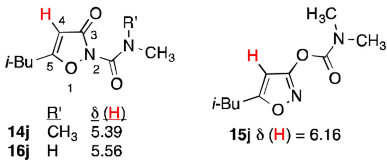
Figure 3. Characteristic chemical shifts of H-4 in 3-oxoisoxazole-2(3 H )-carboxamides and isoxazol-3-yl dimethylcarbamates (ppm), as illustrated by 14j , 16j , and 15j respectively.
