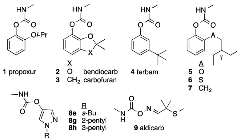
Figure 1. Structure of commercial carbamates ( 1-4, 9 ), and previously reported aryl ( 5-7 ) and pyrazol-4-yl ( 8e, 8g, 8h ) carbamates.
