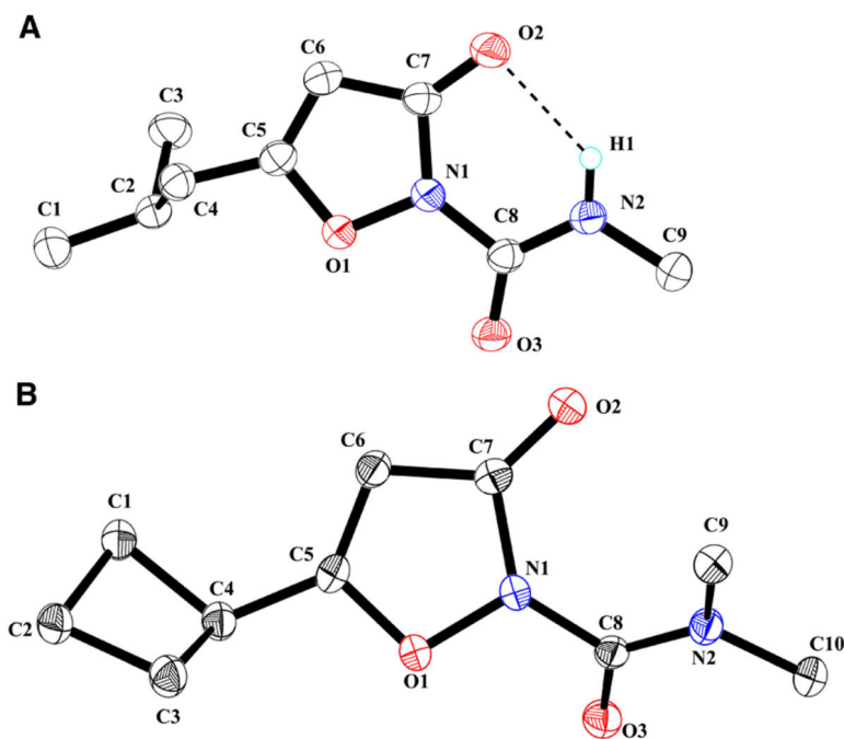
Figure 4. A) Anisotropic displacement ellipsoid drawings (50%) of X-ray structure of compound 16j . Hydrogen atoms were omitted for clarity, except at the exocyclic N . A predicted hydrogen bond is shown with a dotted black line (H1-O2 distance 2.11 Å). B) Anisotropic displacement ellipsoid drawings (50%) of X-ray structure of compound 14d . These structures were deposited at the Cambridge Structural Database (CCDC-1034990 and CCDC-1034991) and were visualized using OLEX2. 17
