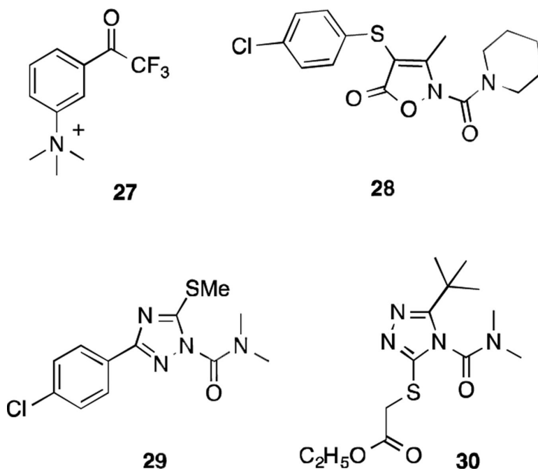
Figure 5. Serine hydrolase inhibitors related to dimethylcarboxamides 14 . 13,22,23
