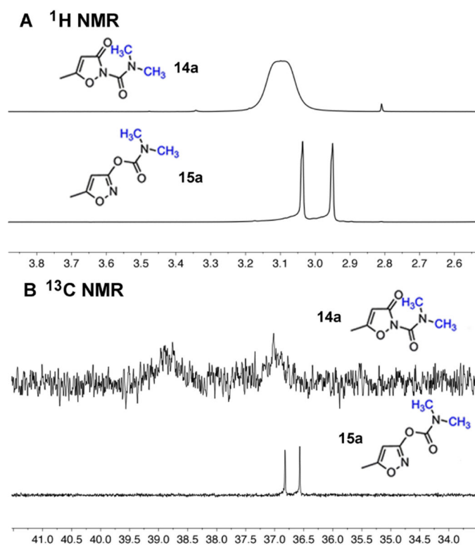
Figure 2. A) The \text{N-Me} regions of the ^1\text{H} NMR spectra of 3-oxoisoxazole-2(3 H )-carboxamide 14a and isoxazol-3-yl carbamate 15a . B) The \text{N-Me} regions of the ^{13}\text{C} NMR spectra of these compounds.
