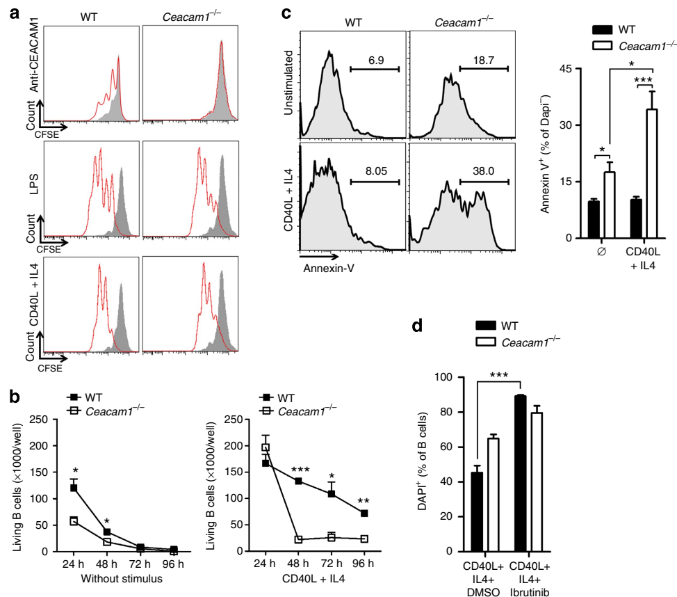
Figure 3 | CEACAM1 promotes survival of B cells in vitro . (a) Representative flow cytometry histogram of proliferating B cells from wild-type (WT) or Ceacam1 -/- mice that were left untreated (grey area) or were further challenged (red line) with anti-CEACAM1 antibody, with LPS, or with recombinant mouse CD40 ligand in combination with mouse IL-4 for 48 h, as determined by FACS analysis. Histograms show DAPI - cells ( n=6 ). (b) Absolute numbers of living B cells (DAPI - ) sorted from spleen and after challenge with or without recombinant mouse CD40 ligand in combination with mouse IL-4 ( n=3 ) determined by FACS analysis. (c) Representative histogram and statistical analysis of Annexin-V + B cells, which were stimulated with recombinant mouse CD40 ligand in combination with mouse IL-4 or were left unstimulated for 48 h (gated on DAPI - B cells, n=6 ). (d) Percentage of DAPI + B cells sorted from spleen of WT and Ceacam1 -/- mice after challenge with recombinant mouse CD40 ligand in combination with mouse IL-4 cultured in the presence or absence of Btk inhibitor Ibrutinib for 48 h determined by FACS analysis ( n=6 ). * P<0.05 ; ** P<0.01 and *** P<0.001 (Student's t -test). Data are representative of one of two (b) or two (a,c,d) experiments (mean \pm s.e.m. (b-d)).
