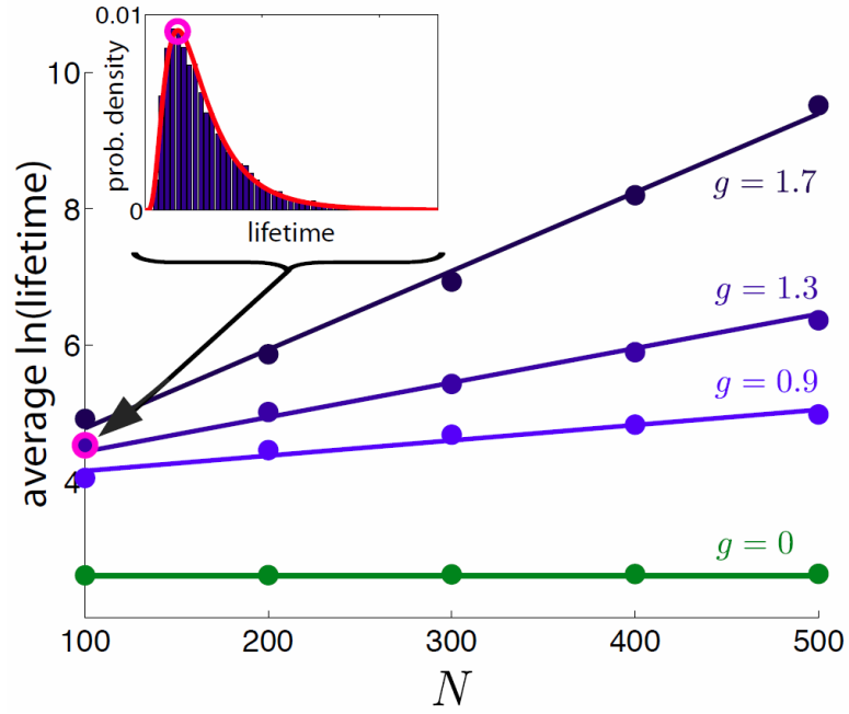
FIG. 5. Exponential dependence on the network size N of the lifetime of the transient activity in the region with stable nonzero fixed points. Inset: Distribution of times to reach a fixed point for N=100 , s=2.3 and g=1.3 , shown with bars. The curve is a fit to a log-normal distribution. Main figure: The average of the logarithm of the time to reach a fixed point plotted as a function of N , for different g values. In all these examples, s = 2.3 . For g = 0 the units are decoupled and the lifetime is independent of N . For g > 0 , the lifetime is exponential in N .
