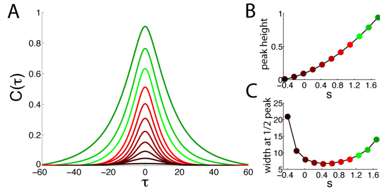
FIG. 4. Autocorrelation functions for different s values and g = 1.5 . A) C(\tau) for, from the top to the bottom curve, s ranging from 1.6 to -0.4 in steps of 0.2. B) Peak heights of the curves in A. C) Widths at 1/2 peak for the curves in A.
