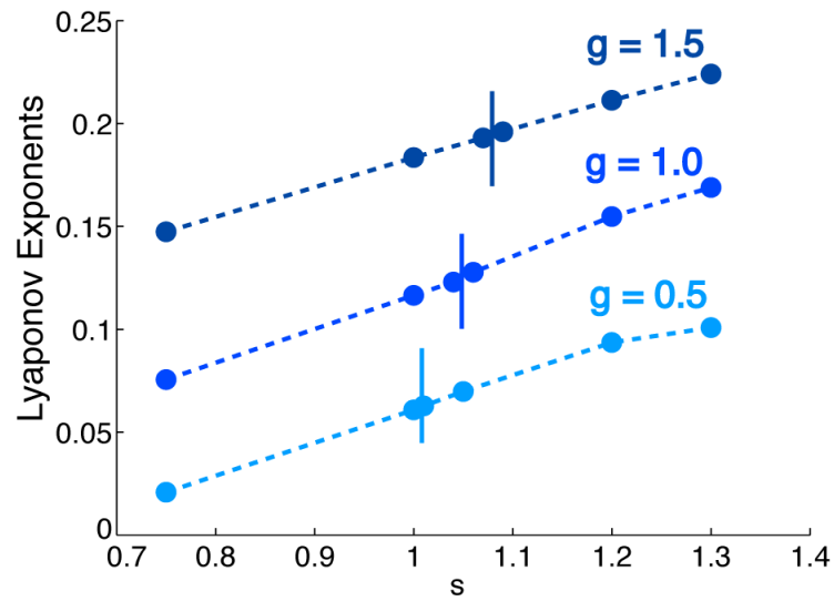
FIG. 6. Maximum Lyapunov exponents as a function of s for three different g values. The vertical lines indicate where the transition from persistent chaos (to the left of these lines) to stable fixed points (to the right) occurs. The maximal Lyapunov exponents vary continuously and smoothly through this transition.
