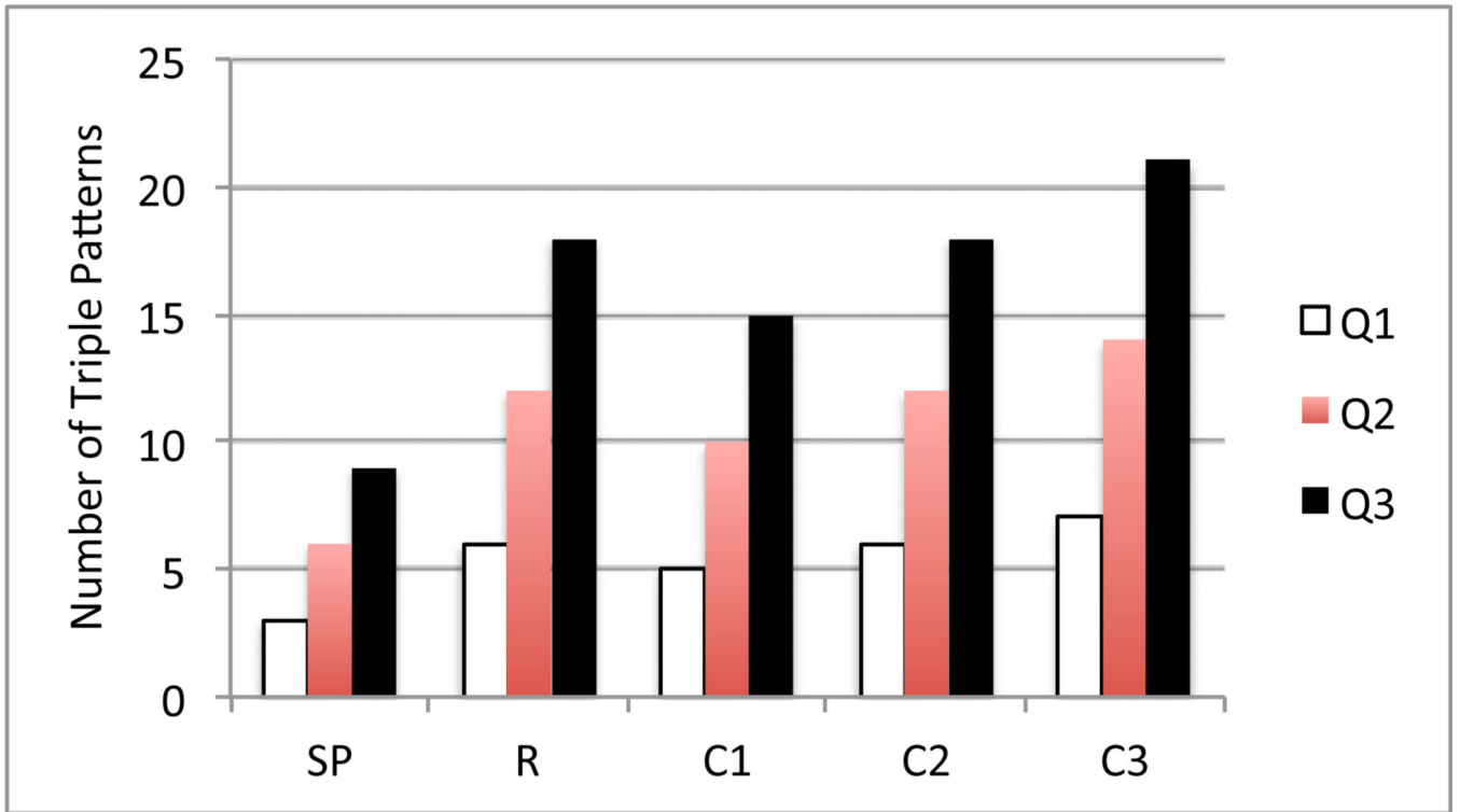
Figure 4. Number of triple patterns within three queries Q1, Q2, and Q3 of query set B.
