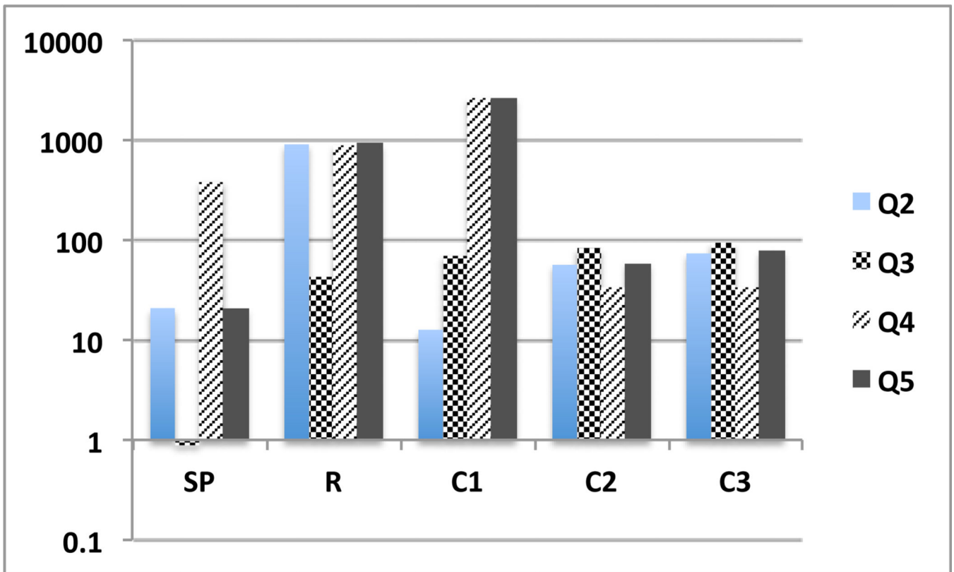
Figure 3. Query performance in msec.: 100 values.
