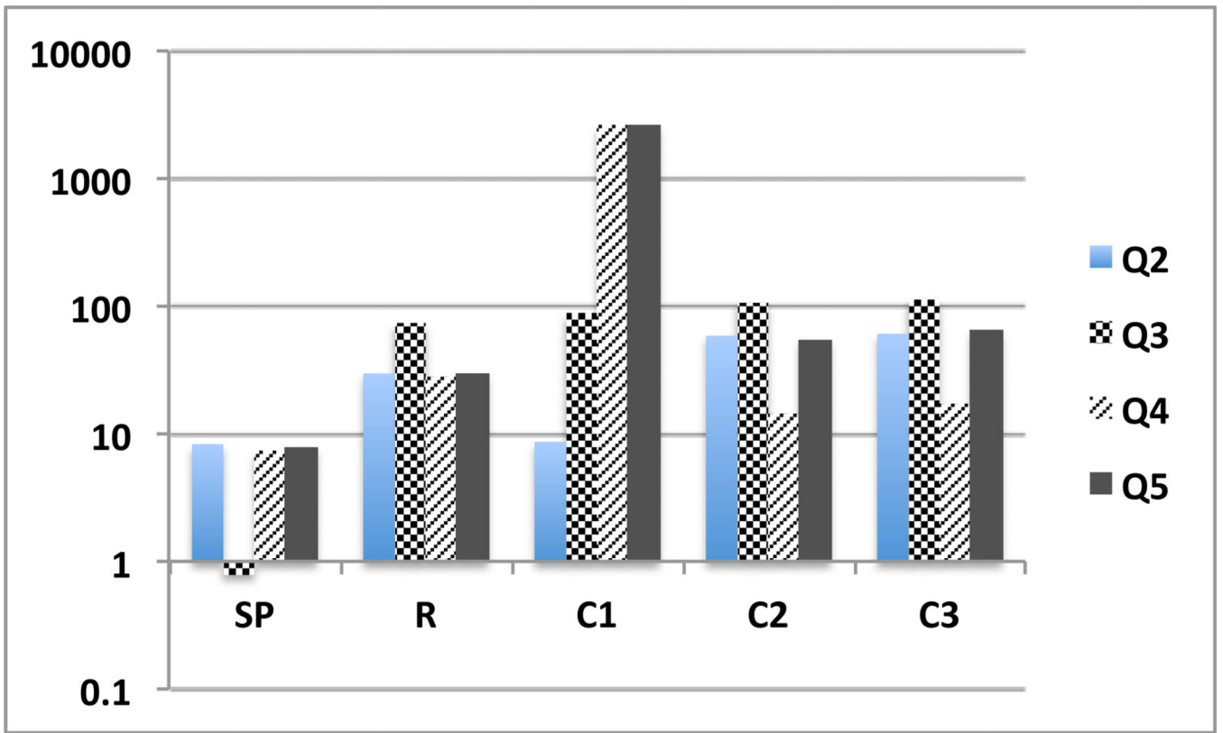
Figure 2. Query performance in msec.: fixed values.
