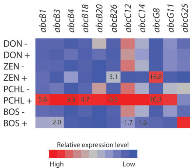
Fig. 7. —Gene expression of selected ABC transporters in C. rosea . Gene expression of ABC transporters was assayed by RT-qPCR during exposure of C. rosea to deoxynivalenone (DON+), zearalenone (ZEN+), Boscalid (BOS+) and P. chlororaphis metabolites (PCHL+), and compared with the corresponding control (–). Relative expression levels are color-coded. Statistically significant ( P \leq 0.05 ) changes are indicated by fold change numbers.
