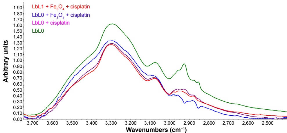
Figure 7 Fourier transform infrared spectra of the samples. Abbreviations: LbL, layer-by-layer; Fe_3O_4 , magnetite.
