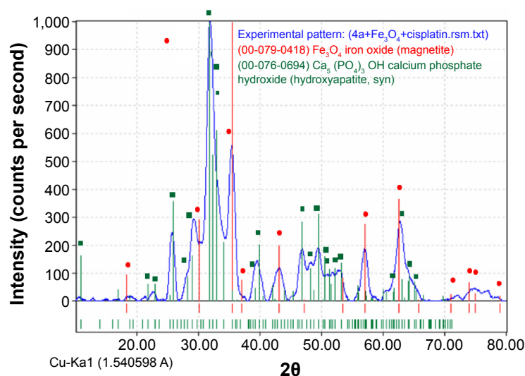
Figure 1 X-ray diffraction pattern of COLL/HA-Fe 3 O 4 -CisPt composite material obtained for a sample with seven layers. Abbreviations: COLL, collagen; HA, hydroxyapatite; Fe 3 O 4 , magnetite; CisPt, cisplatin.
