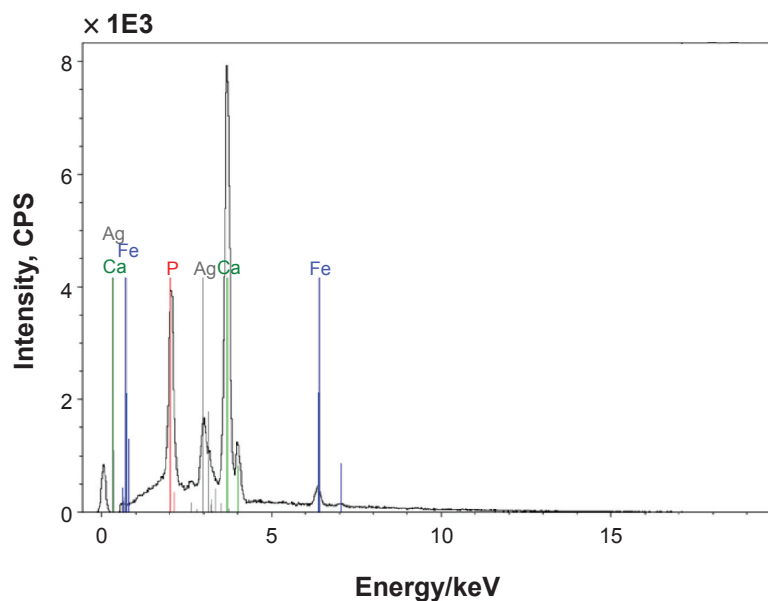
Figure 6 Elemental assignment of the energy-dispersive X-ray spectroscopy peaks (COLL/HA- Fe_3O_4 -CisPt obtained for a sample with seven layers). Abbreviations: COLL, collagen; HA, hydroxyapatite; Fe_3O_4 , magnetite; CisPt, cisplatin; CPS, counts per second.
