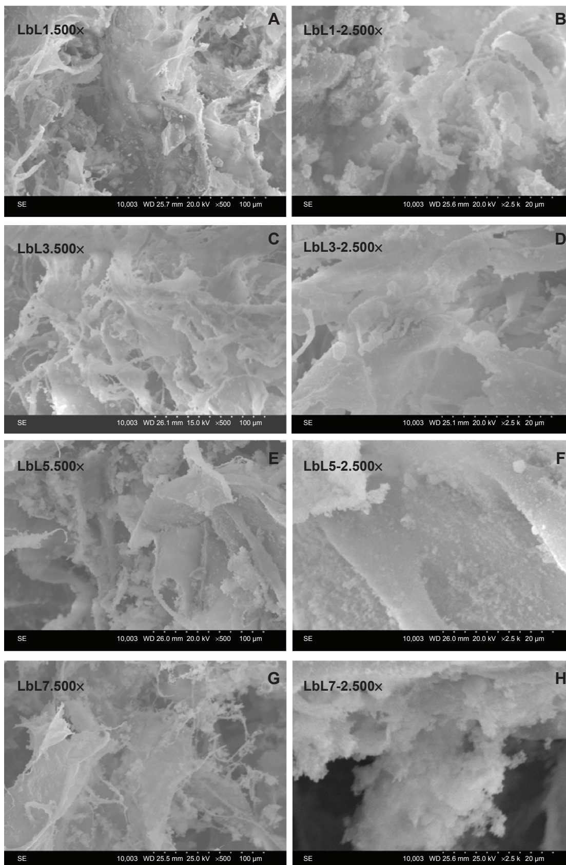
Figure 5 Scanning electron microscopy images of COLL/HA-Fe 3 O 4 -CisPt obtained using a layer-by-layer technique (one, three, five, and seven layers).
