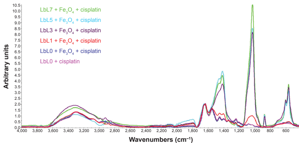
Figure 8 Fourier transform infrared spectra of the different samples containing collagen, hydroxyapatite, magnetite, and cisplatin. Abbreviations: LbL, layer-by-layer; Fe_3O_4 , magnetite.
