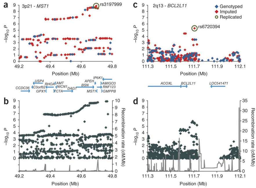
Figure 1. Association results at the MST1 and BCL2L11 loci. (a,c) The association results from the genotyped and imputed markers at the MST1 and BCL2L11 loci are shown as the -\log_{10} of the P values plotted against the genomic position (NCBI build 36). The MST1 and BCL2L11 SNPs with robust evidence for replication are highlighted with green circles. (b,d) The recombination rates (gray lines) derived from the HapMap project, along with the association results based on an imputed dataset using reference data from the 1000 Genomes Project. None of the imputed 1000 Genomes Project SNPs in the region from 111,745,000 bp to 111,929,500 bp on chromosome 2 passed imputation quality thresholds (Supplementary Methods). The MST1 and BCL2L11 associations (represented by the SNPs given in Table 1) were independent of the HLA association in a logistic regression analysis with inclusion of rs3134792 (the most strongly associated HLA SNP) as a covariate and in a stratified analysis according to rs3134792 risk allele carriership (Supplementary Table 2). Association results at the MST1 and BCL2L11 loci in ulcerative colitis compared to PSC are shown in Supplementary Figure 3.
