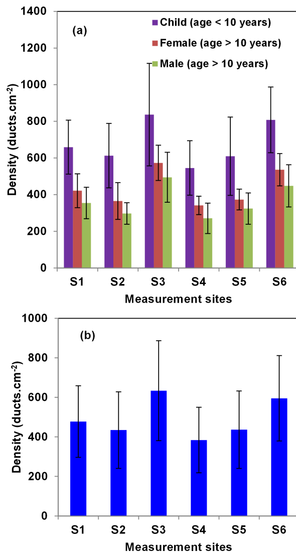
Figure 2 | (a) Variation in ensemble averaged duct density at different measurement sites in subjects of different ages and gender. (b) Sweat duct density variation in ensemble averaged over all subjects. In both cases the error bars represents the standard deviation in the sample pool.
