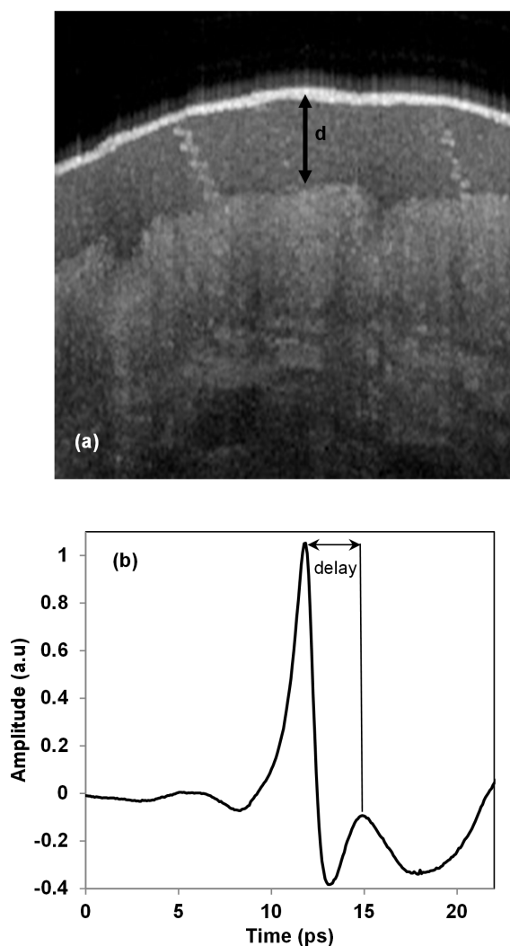
Figure 4 | (a) Thickness ( d ) of the stratum corneum. (b) THz time-domain pulse reflected from the palm of the hand.
