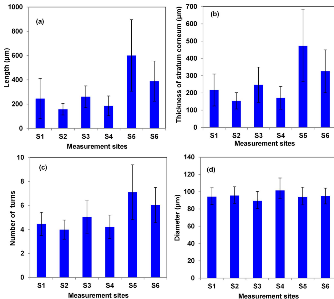
Figure 3 | (a) Lengths of the ducts and their standard deviations. (b) Thickness of the stratum corneum and their standard deviation. (c) Number of turns and their standard deviations (d) Diameter of the sweat ducts and their standard deviation
