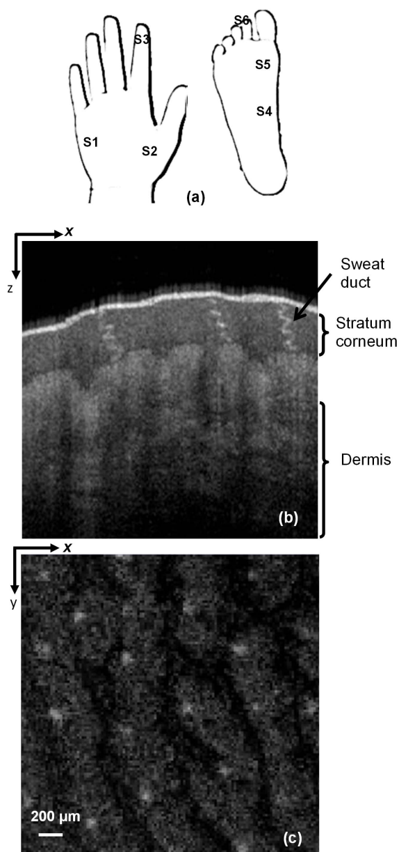
Figure 1 | (a) Imaging sites where S1: Base of little finger; S2: Between thumb and wrist; S3: Index finger tip; S4: Inner arch; S5: Mound of big toe; S6: Right second toe (b) Typical optical coherence tomography (OCT) image in the x-z plane showing the stratum corneum, sweat duct and dermis (c) A 2.5 × 2.5-mm en face OCT image in the x-y plane showing the sweat gland duct distribution. Here, the light white spots are the sweat ducts and the light gray features are due to the undulations of the skin surface (fingerprints).
