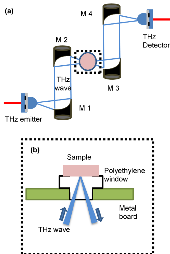
Figure 5 | (a) A schematic of the experimental setup for the THz wave reflection measurements. (b) Side view of the dotted box in Fig. 5a.
