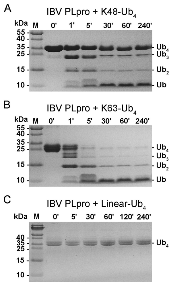
FIGURE 4. Cleavage of polyubiquitin chains by PLpro from IBV. A , picture of the gel from SDS-PAGE analysis of reaction products of Lys 48 -linked tetraubiquitin chains treated with IBV PLpro at different time intervals. B , analysis similar to that in A except the substrate used was Lys 63 -linked tetraubiquitin. C , SDS-PAGE gel picture of reaction products of linear ubiquitin chains treated with PLpro from IBV. The protease could not cleave linear ubiquitin under reaction conditions similar to those used for cleaving Lys 48 - and Lys 63 -linked tetraubiquitin. M , molecular mass markers; t , minutes.
