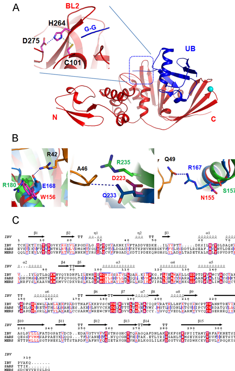
FIGURE 3. Substrate binding site of IBV PLpro. A , ubiquitin (UB; blue schematic) from the structure of PLpro of SARS CoV bound with ubiquitin (Protein Data Bank code 4M0W) was superimposed over the structure of PLpro from IBV (red schematic). The location of the diglycine motif (G-G) with respect to the catalytic triad (shown as sticks) and BL2 is shown (inset). Interaction between the catalytic residues is shown by dashed lines. B , comparison of amino acids of different PLpros interacting with ubiquitin (orange color). Interactions of amino acids of ubiquitin such as Arg 42 , Ala 46 , and Gln 49 (orange sticks) with corresponding amino acids of the PLpro from IBV (magenta sticks), SARS (blue sticks), and MERS (green sticks) CoVs are shown to illustrate the differences in residues of the ligand binding site of the PLpros from different sources. C , alignment of primary sequences of PLpro from IBV, SARS, and MERS CoVs. Secondary structural elements of PLpro from IBV are shown at the top. Absolutely conserved residues are highlighted with a red background. Conserved residues are shown in red.
