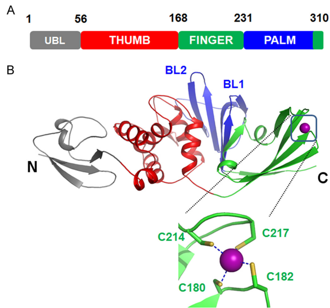
FIGURE 1. Overall structure of PLpro from IBV. A, diagrammatic representation of the organization of domains of IBV PLpro inferred from the crystal structure. B, schematic representation of the crystal structure of IBV PLpro. The locations of BL1 and BL2 as well as the termini of the protein are marked. Zn 2+ ion bound by the protein is shown as a sphere. The Zn 2+ ion is coordinated by four cysteine residues (inset) shown as sticks.
