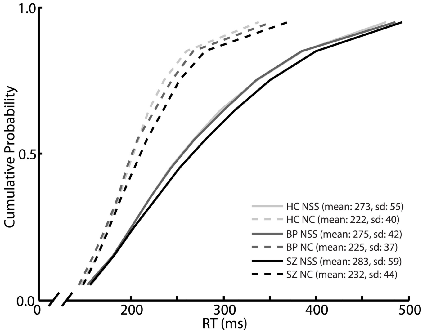
Figure 2. RT distributions
