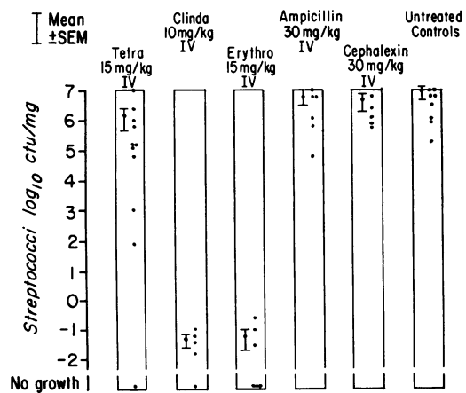
FIGURE 6 Results of quantitative cultures of endocardial vegetations from rabbits with left heart vegetations after multiple-dose 12-hourly antibiotic prophylaxis using an inoculum of log 10 8.0 cfu S. sanguis .
