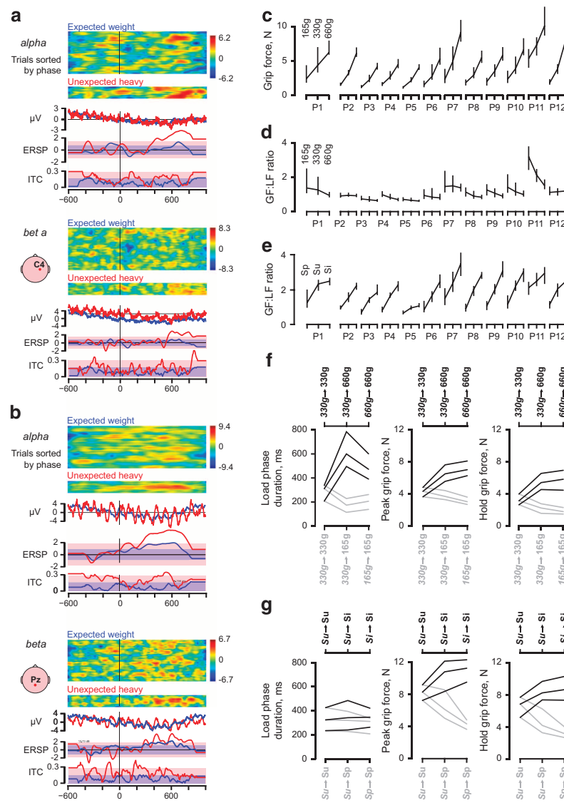
Figure 3. Data validation. (a,b) For channels C4 and Pz (shown in insets) recorded in Participant 3, trials when the object's weight was the same as in the previous trial ( Expected weight , n = 105 ; blue lines) and unexpectedly heavy ( n = 30 ; red lines) were contrasted using EEGLab 11 . The panels show from top, the power in the alpha and beta bands after sorting the trials by phase at the peak frequency, the average EEG amplitudes, the ERSPs and the ITCs. The colored patches represent 95% confidence intervals. The earliest moment this participant on average could have detected an increased object weight was \sim 200 ms after object contact (i.e., time zero). (c) All participants adapted their grip force to the object's weight, i.e., 165, 330 or 660 g in series with sandpaper surfaces. The different weights thus invoked markedly different fingertip forces in all participants. (d) The grip:load force ratio was the same or declined across the three object weights in all participants, i.e., the force coordination was roughly the same irrespective of the object's weight. (e) In series with the same object weight (330 g) but with contact plates covered with sandpaper, suede or silk, the grip:load force ratio increased with decreasing friction, i.e., in all participants the three contact plates offered different object-fingertip friction and all participants adapted to the prevailing friction. (f,g) When the weight (f) or the contact surfaces (g) was unexpectedly changed between trials, there was a marked change in the load force duration, in the peak grip force and the hold grip force (e.g., all increased when the object had an unexpected increased weight or decreased friction). Data aggregated across all participants. The lines represent the median and the 1st and 3rd quartile, black lines increased weight (f) and increased slipperiness (g) and gray lines decreased weight and slipperiness, respectively, as indicated on the top and bottom axes.
