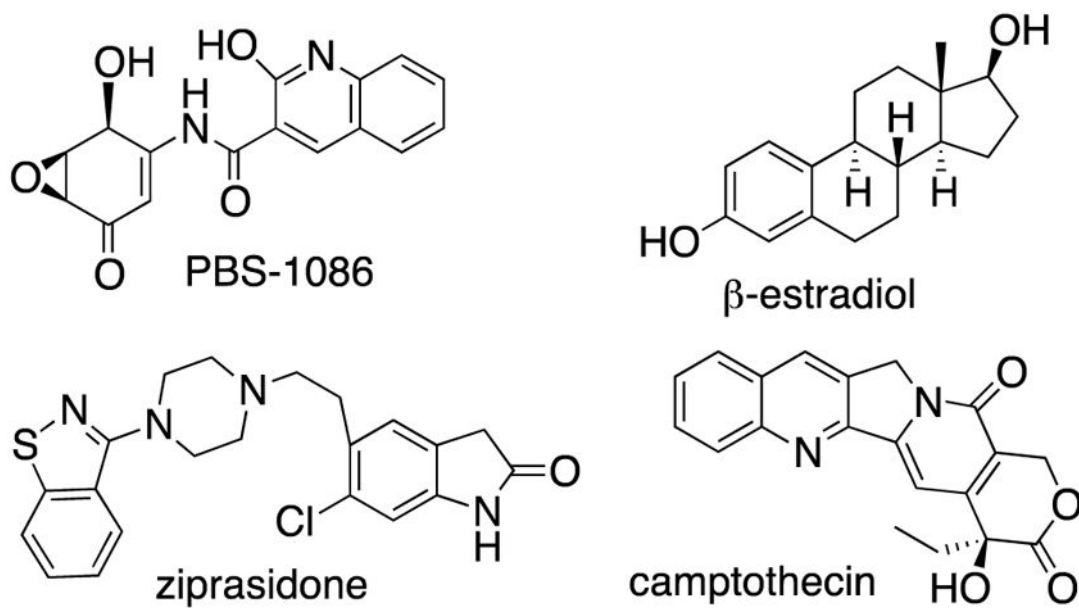
Figure 2. Structures of insoluble drugs used in this study.
