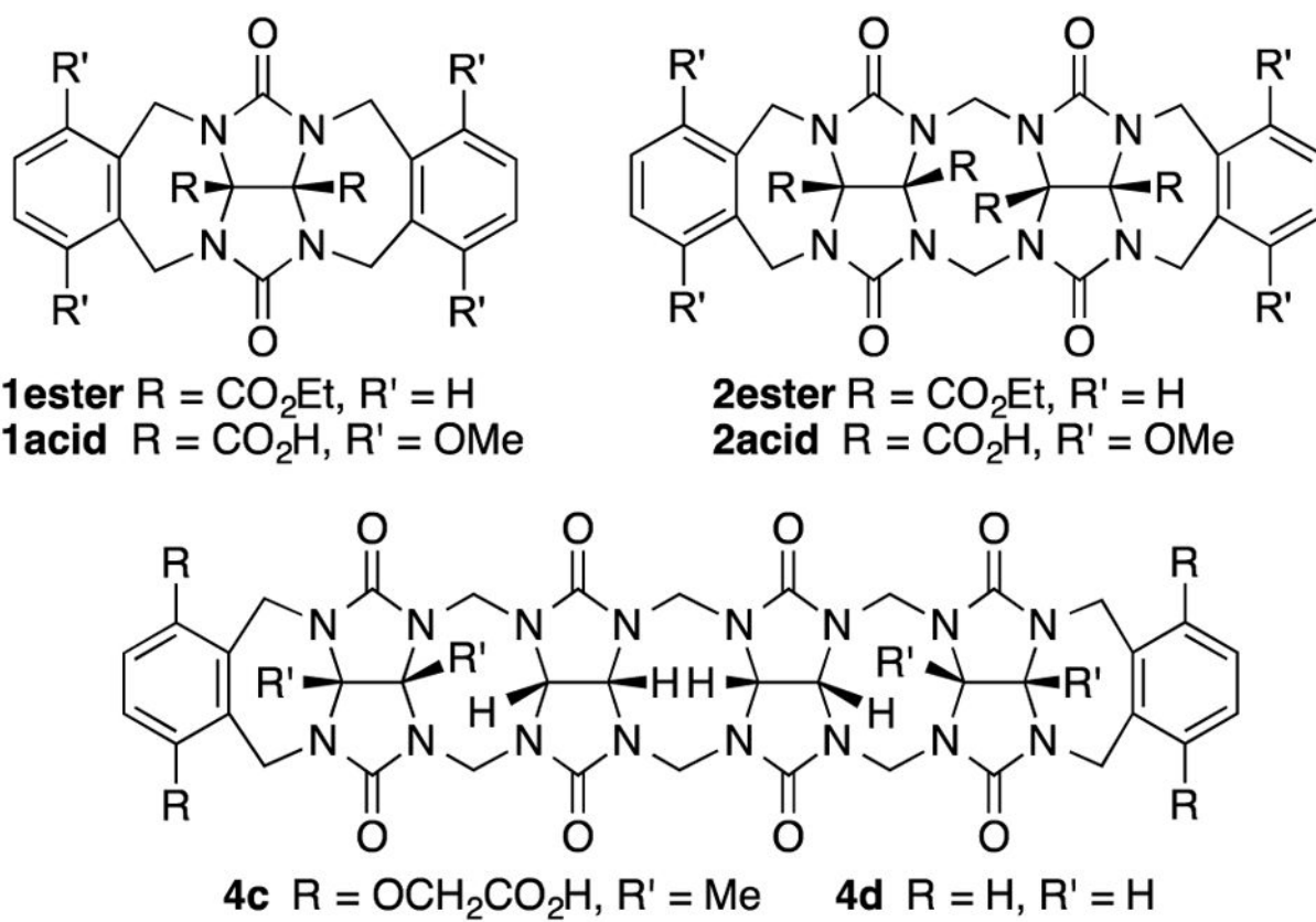
Figure 4. Structures of comparison compounds.
