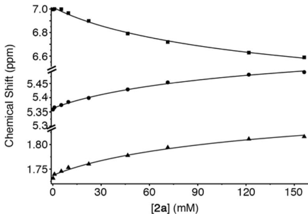
Figure 6. Plot of chemical shift versus [2a]. The solid line represents the best global fit of the data to a two-fold self-association model with K_s = 12 \text{ M}^{-1} . Conditions: 20 mM sodium phosphate buffered \text{D}_2\text{O} , pD 7.4, room temperature. Key: H a , ■; H b , ●; H c , ▲.
