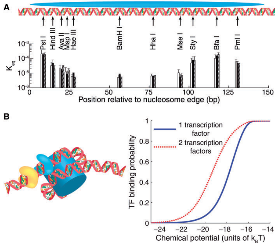
Figure 3: DNA accessibility and TF binding to nucleosomal DNA. (A) Restriction enzyme sites inserted into the 60I nucleosome sequence at locations indicated by black arrows [56]. Each group of three bars represents independent measurements in which the 60I sequence was flanked by different DNA sequences. The height of each bar is the equilibrium constant K_{eq} for site exposure averaged over multiple experiments; error bars show standard deviations. (B) Nucleosome-induced cooperativity between two DNA-binding factors. Left panel: two TFs bound simultaneously to nucleosomal DNA; the nucleosome is partially unwrapped. Right panel: TF binding probability at a site located at bp 31–40 from the edge of the fully wrapped nucleosome, in the absence (blue, solid) or presence (red, dotted) of a second site for the same TF located on the same side of the dyad, at bp 11–20. The free energy of a fully wrapped nucleosome is \ln(10^{-9})k_B T ; histone chemical potential is \ln(10^{-6})k_B T ; TF binding energy is \ln(10^{-10})k_B T for its cognate sites and \ln(10^{-6})k_B T for all other sites [57]. The model of nucleosome unwrapping is as described in [42]. (A colour version of this figure is available online at: http://bfg.oxfordjournals.org )
