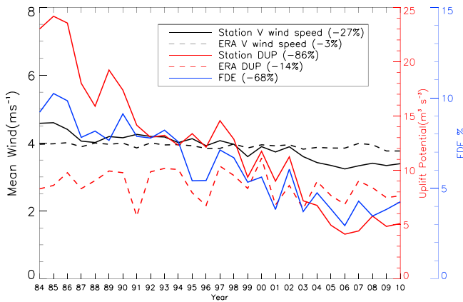
Figure 2. Trends in mean annual 10 m wind speed ( V , black lines), dust uplift potential ( DUP , red lines), and frequency of dust events ( FDE , blue line) from observations averaged over seven surface stations in the Sahel (see Figure 1 for locations; solid lines) and ERA-Interim reanalysis averaged over the blue box shown in Figure 1 (dashed lines) for the time period 1984–2010. Numbers in brackets in the legend indicate the relative change over the time period estimated from the linear trend line as in Table 1. Definitions of DUP and FDE are given in section 2. Note that there is no FDE from reanalysis data. A fixed threshold of 7 \text{ ms}^{-1} was used for the DUP computations.
