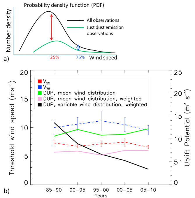
Figure 3. (a) Schematic illustrating the estimation of emission threshold wind velocities using probability density distributions for all wind observations and those during dust emission events. Probabilities of 25% ( v_{25} ) and 75% ( v_{75} ) were arbitrarily selected to characterize the range of wind speeds typical for the beginning of dust emission. (b) Time evolution of v_{25} and v_{75} threshold velocities computed for each station, for 5 year periods from 1985–2010, then averaged over all stations (dashed lines, left axis). Standard deviations of v_{25} and v_{75} wind speeds are given by the error bars. Corresponding DUP calculations are also shown (right axis) using (1) a mean wind distribution over the whole time period and the v_{25} threshold velocity (green), (2) a mean wind distribution and a probability weighting (purple), and (3) a varying wind distribution representative of each 5 year period and a probability weighting (black).
