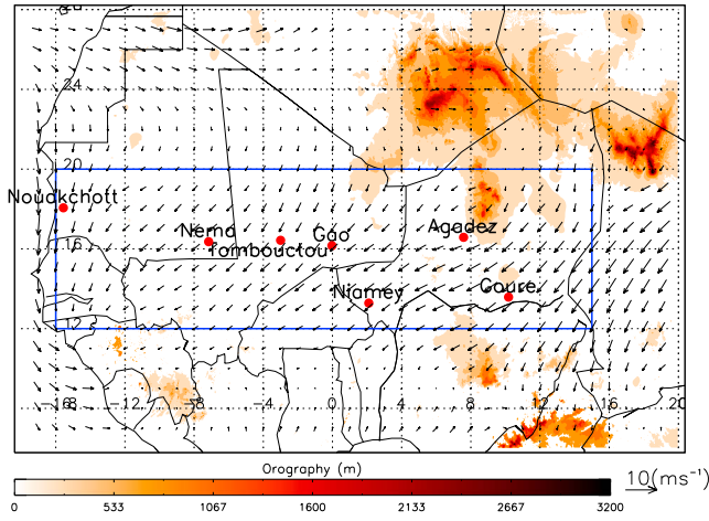
Figure 1. Map showing the location of the seven Sahelian stations used in this study (red dots with labels), the orography (shaded in m above mean sea level according to the legend), and the domain used for averaging ERA-Interim reanalysis data in blue. Winter mean (December–February) 10 m wind vectors from ERA-Interim are also included (scale in bottom right corner).
