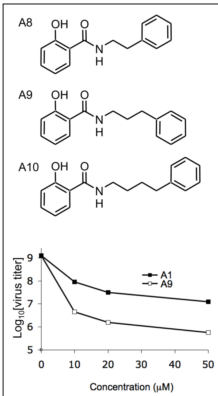
Figure 3. Ortho hydroxybenzamide analogs
