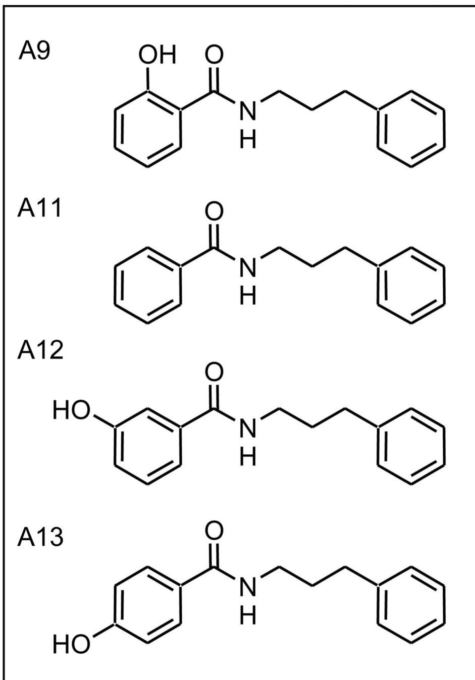
Figure 4. Benzamide analogs
