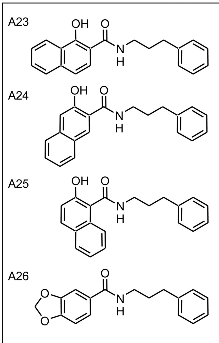
Figure 6. Naphthoic acid analogs
