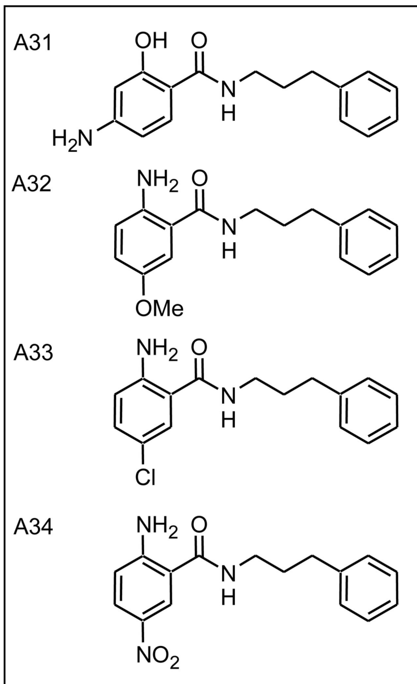
Figure 8. Disubstituted benzamide analogs
