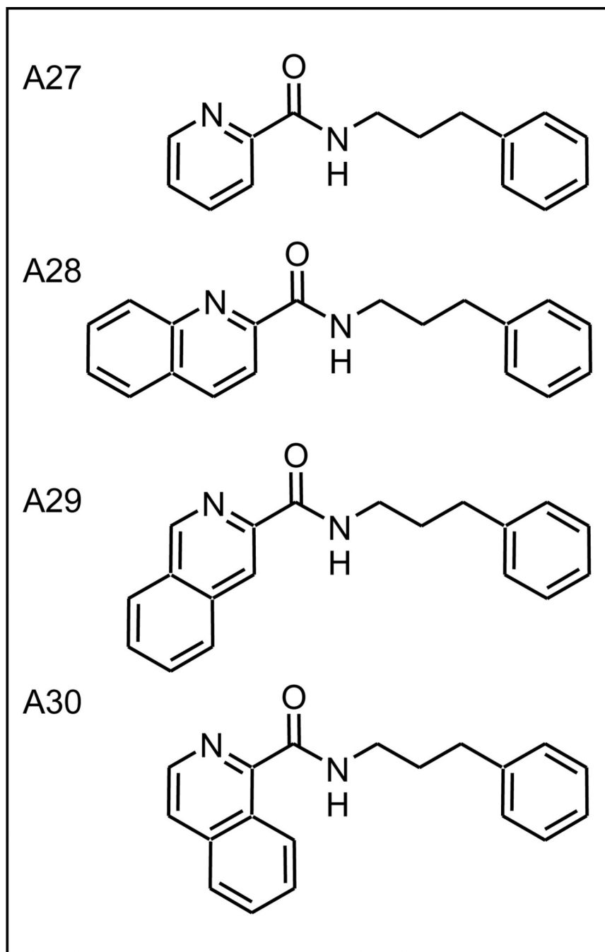
Figure 7. Pyridyl analog A27 and Quinolylnyl analogs A28 – A30
