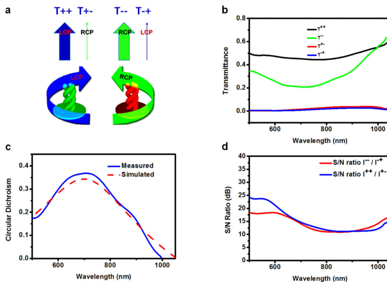
Figure 3. Circular dichroism and S/N ratio
