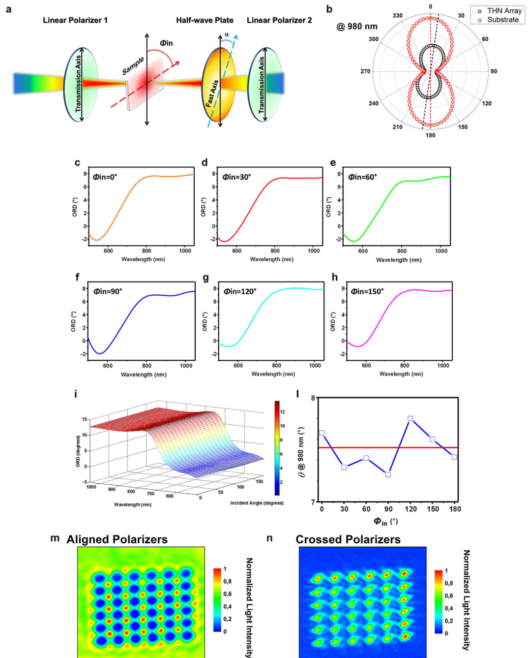
Figure 4. Optical Rotatory Dispersion and Circular Birefringence
