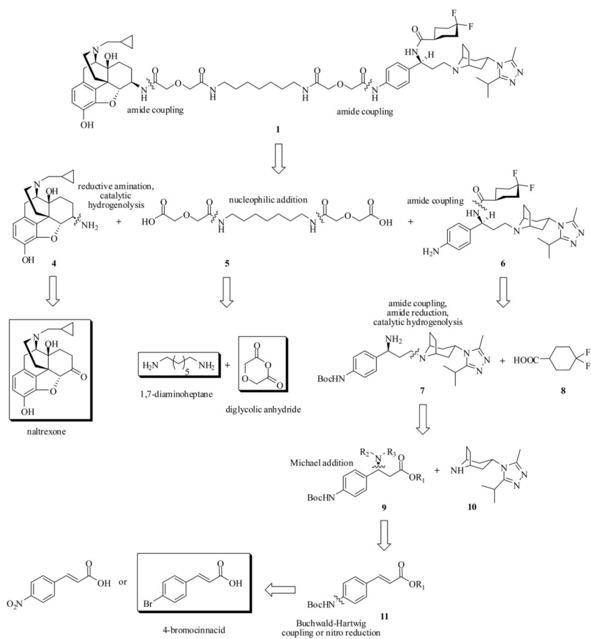
Scheme 1. Retrosynthetic analysis of the bivalent ligand 1
