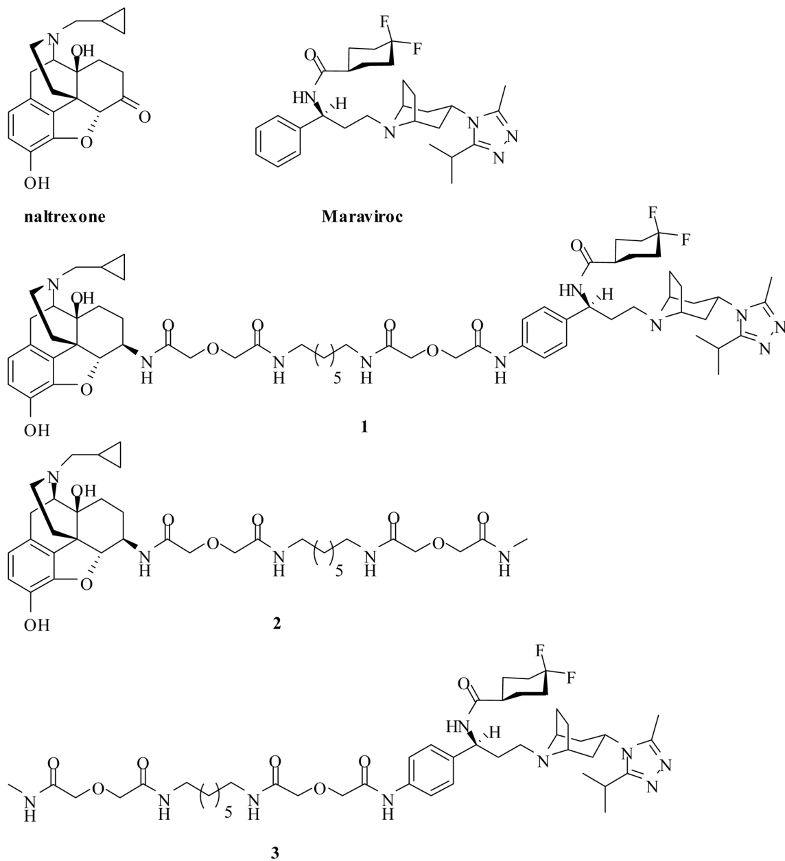
Figure 1. Chemical structures of naltrexone, Maraviroc, designed bivalent ( 1 ) and monovalent ligands ( 2 , 3 ).
