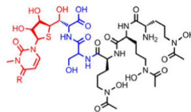
Albomycin ε R = \text{NH} Albomycin δ 1 R = \text{O} Albomycin δ 2 R = \text{N} \begin{array}{c} \text{O} \\ \parallel \\ \text{NH}_2 \end{array}
