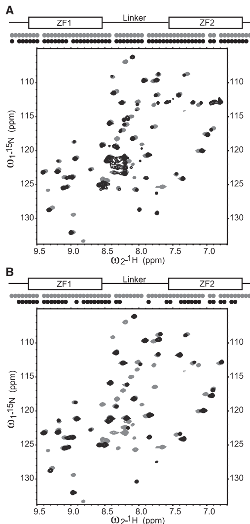
FIGURE 2 Comparison of ^{15}\text{N} - ^1\text{H} HSQC spectra. Dots on top of the spectrum indicate whether a crosspeak was observed for each residue. (A) TIS11d (gray) and TIS11d-E220A (black), (B) TIS11d (gray) and TIS11d- \Delta D219/E220 (black).
