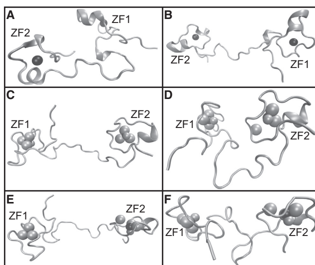
FIGURE 6 Example structures of TIS11d-E220A (A and B) and TIS11d-Δ D219/E220 (C–F). Black spheres: zinc ions, gray spheres: sulfur atoms of coordinating cysteine residues ( large spheres ) and nitrogen residues ( small spheres ), gray ribbon: backbone. TIS11d-E220A: (A) before extension, (B) during extension. TIS11d-Δ D219/E220: (C) extension with zinc ion of ZF2 still coordinated to Cys-212, (D) after extension with loss of Cys-212 coordination, (E) extended structure with loss of Cys-212 coordination, (F) more compact structure with crossed linker structure.
