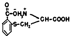
Salt linkage
