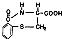
Amide linkage
